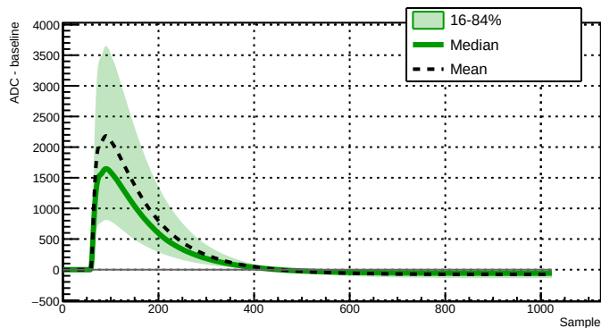
Run 039518 - Channel 2080 - 27811 waveforms
