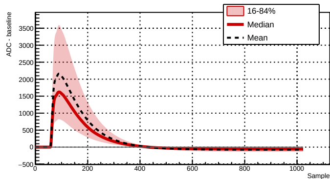
Run 039518 - Channel 2081 - 28211 waveforms
