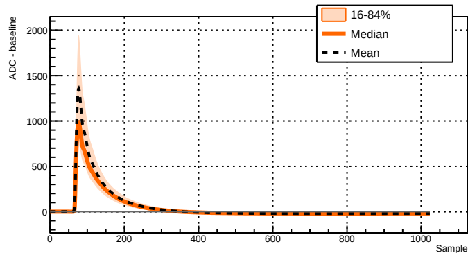
Run 039518 - Channel 2071 - 11437 waveforms
