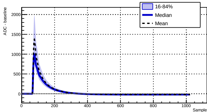
Run 039518 - Channel 2070 - 11703 waveforms
