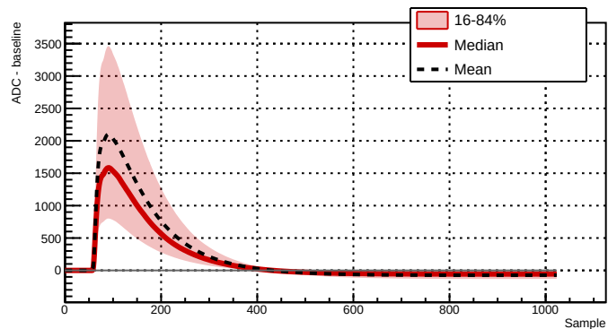
Run 039519 - Channel 2081 - 27788 waveforms
