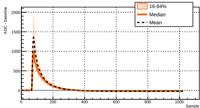
Run 039519 - Channel 2071 - 11080 waveforms
