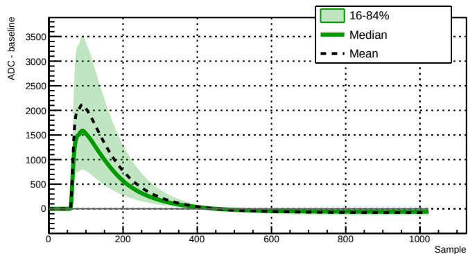
Run 039519 - Channel 2080 - 27661 waveforms
