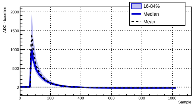
Run 039519 - Channel 2070 - 11516 waveforms
