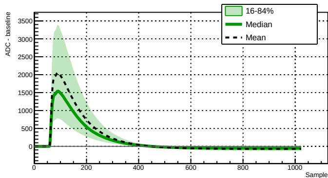
Run 039521 - Channel 2080 - 26836 waveforms
