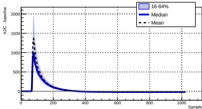
Run 039521 - Channel 2070 - 10974 waveforms
