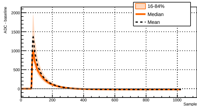
Run 039521 - Channel 2071 - 10491 waveforms
