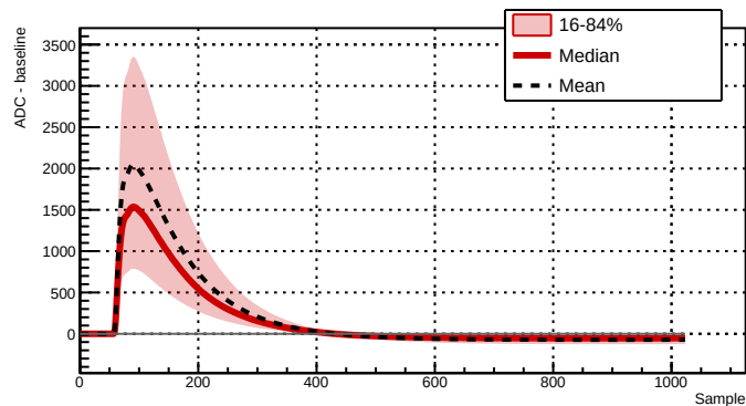
Run 039521 - Channel 2081 - 26942 waveforms
