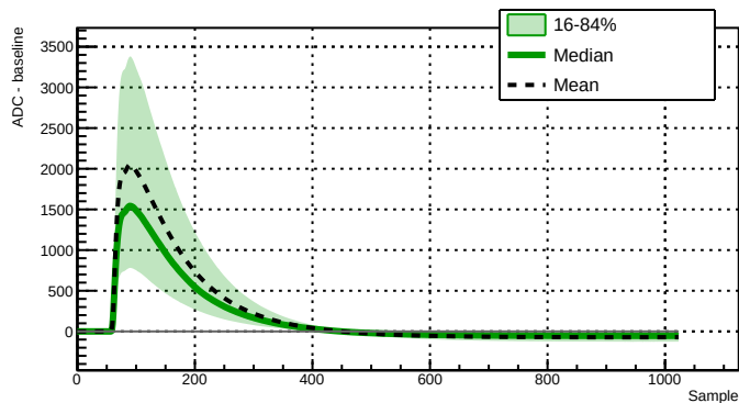
Run 039522 - Channel 2080 - 26496 waveforms
