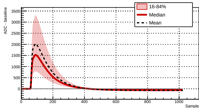
Run 039522 - Channel 2081 - 26780 waveforms
