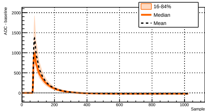
Run 039522 - Channel 2071 - 10202 waveforms
