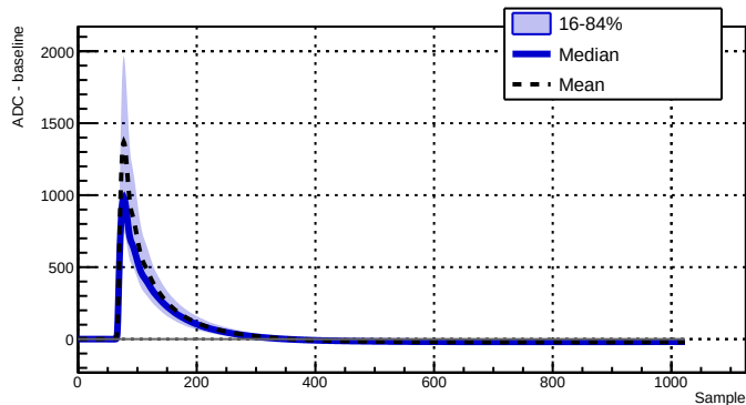
Run 039522 - Channel 2070 - 10691 waveforms
