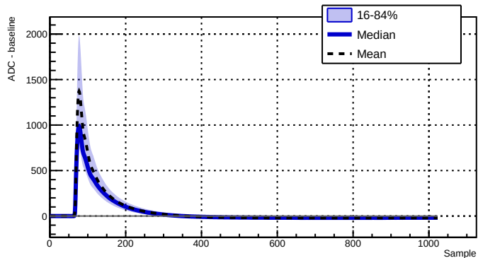
Run 039523 - Channel 2070 - 10057 waveforms
