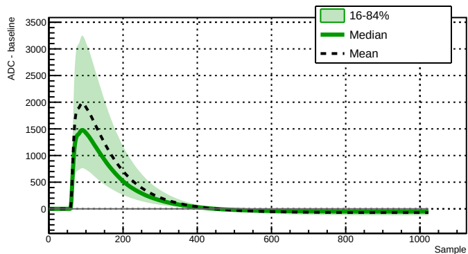
Run 039523 - Channel 2080 - 25977 waveforms
