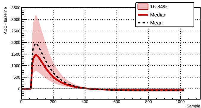
Run 039523 - Channel 2081 - 26179 waveforms
