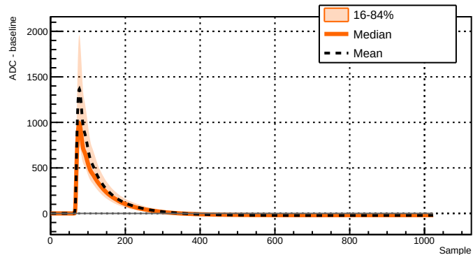
Run 039525 - Channel 2071 - 9490 waveforms
