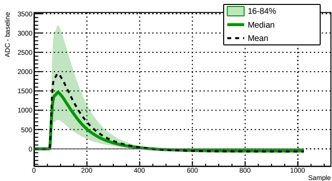
Run 039525 - Channel 2080 - 25594 waveforms
