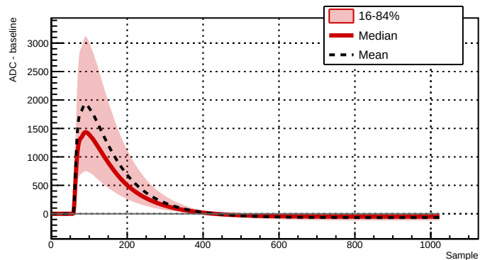
Run 039525 - Channel 2081 - 25782 waveforms
