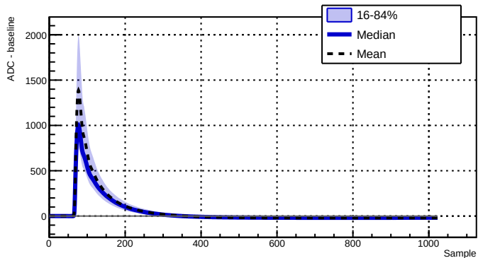
Run 039525 - Channel 2070 - 9733 waveforms
