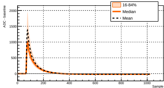
Run 039528 - Channel 2071 - 8714 waveforms
