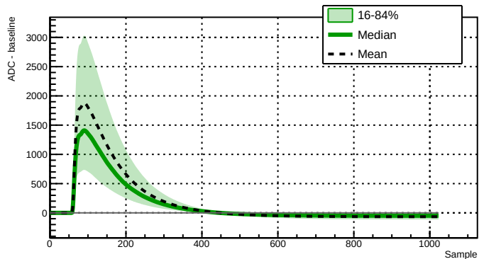
Run 039528 - Channel 2080 - 25012 waveforms
