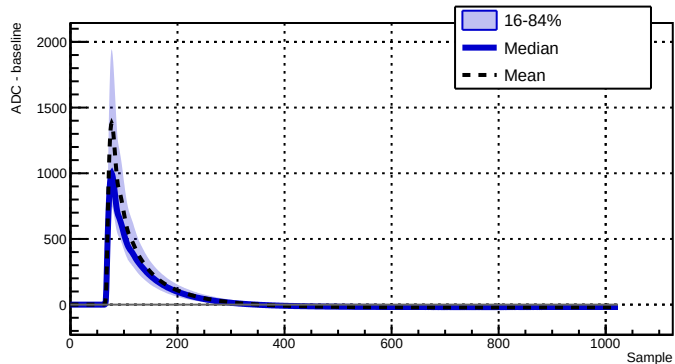
Run 039528 - Channel 2070 - 9107 waveforms
