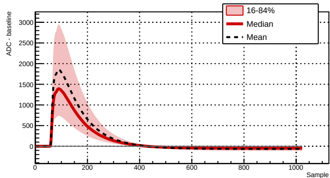
Run 039528 - Channel 2081 - 25065 waveforms
