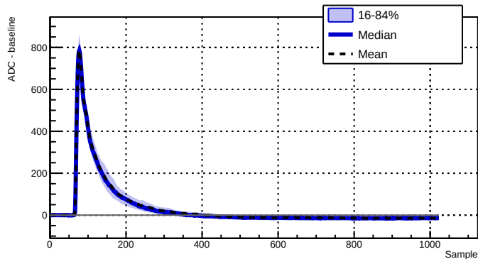
Run 040931 - Channel 2070 - 232 waveforms
