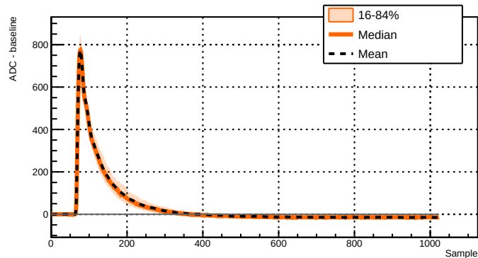
Run 040931 - Channel 2071 - 223 waveforms
