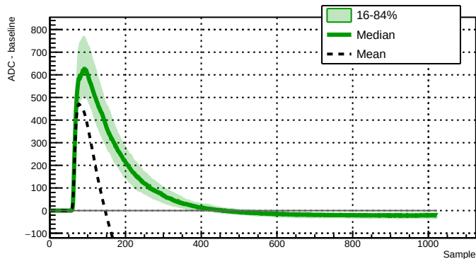
Run 040931 - Channel 2080 - 385 waveforms
