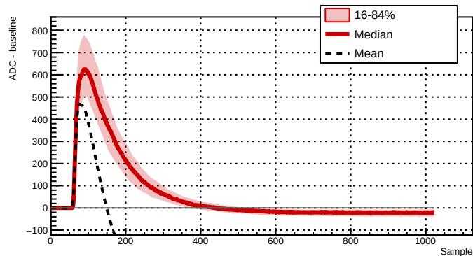
Run 040931 - Channel 2081 - 413 waveforms
