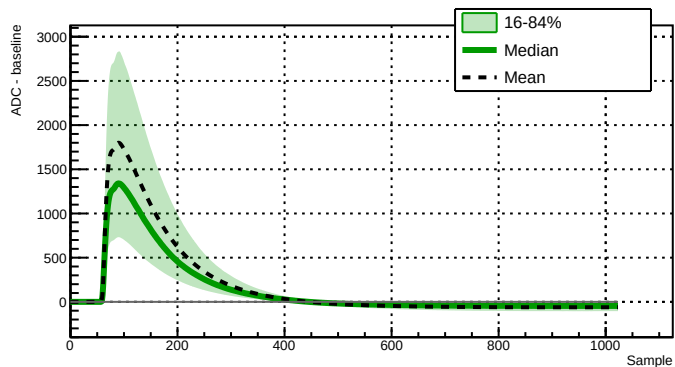
Run 043383 - Channel 2080 - 20268 waveforms
