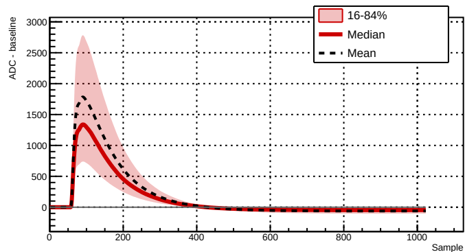
Run 043383 - Channel 2081 - 20242 waveforms
