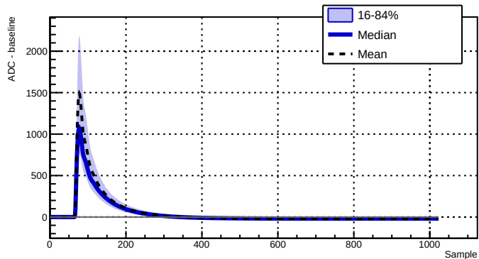
Run 043383 - Channel 2070 - 6948 waveforms
