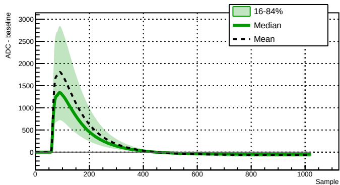
Run 043384 - Channel 2080 - 20352 waveforms
