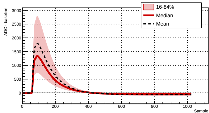
Run 043384 - Channel 2081 - 20465 waveforms
