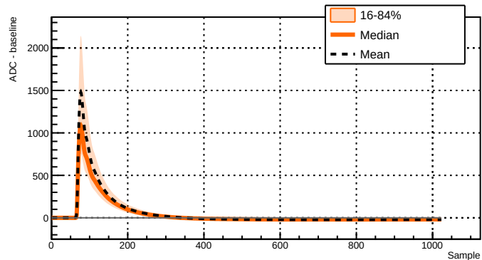
Run 043384 - Channel 2071 - 6937 waveforms
