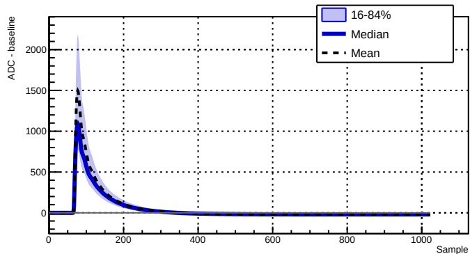
Run 043384 - Channel 2070 - 7091 waveforms
