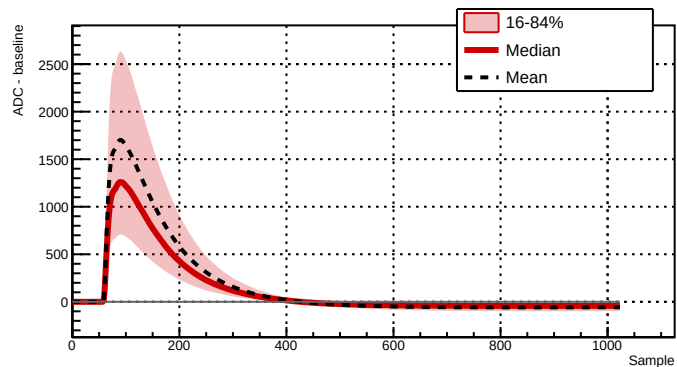
Run 043387 - Channel 2081 - 18747 waveforms
