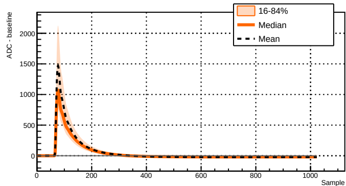
Run 043387 - Channel 2071 - 6016 waveforms
