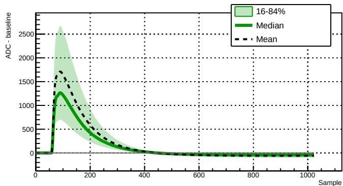
Run 043387 - Channel 2080 - 18853 waveforms
