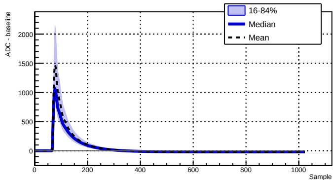
Run 043387 - Channel 2070 - 6236 waveforms
