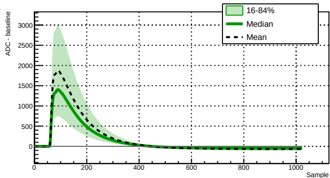
Run 043389 - Channel 2080 - 21822 waveforms
