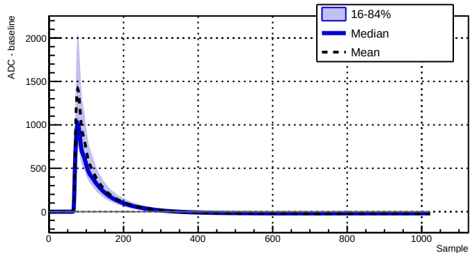
Run 043389 - Channel 2070 - 7829 waveforms
