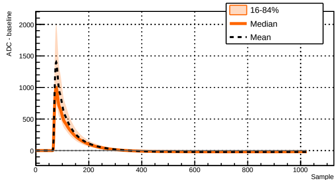
Run 043389 - Channel 2071 - 7616 waveforms
