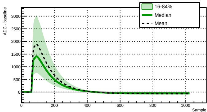
Run 043390 - Channel 2080 - 21800 waveforms
