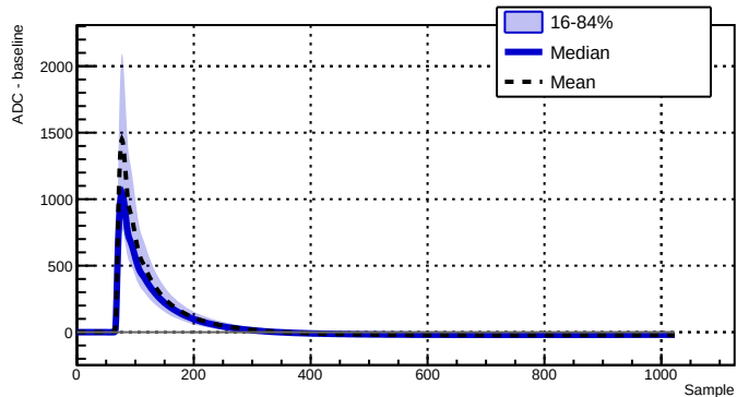
Run 043390 - Channel 2070 - 7748 waveforms
