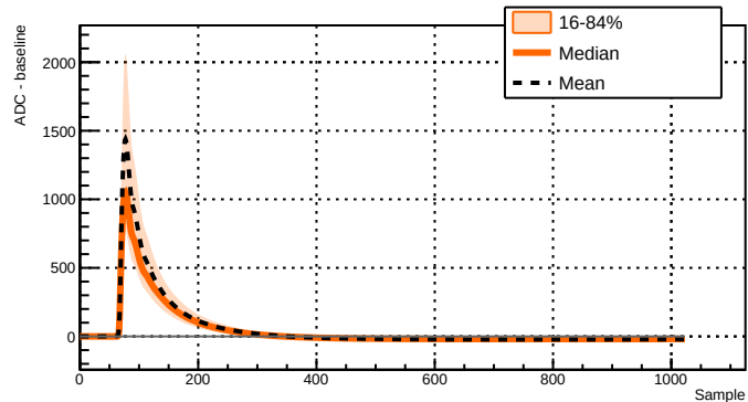
Run 043390 - Channel 2071 - 7540 waveforms
