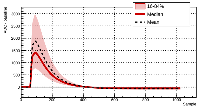
Run 043390 - Channel 2081 - 21802 waveforms
