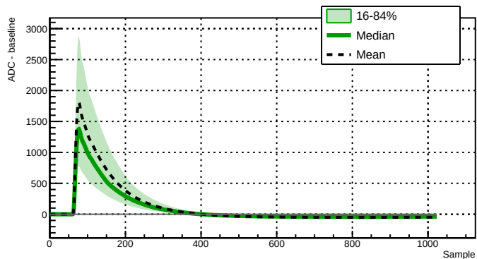
Run 039500 - Channel 2060 - 7310 waveforms
