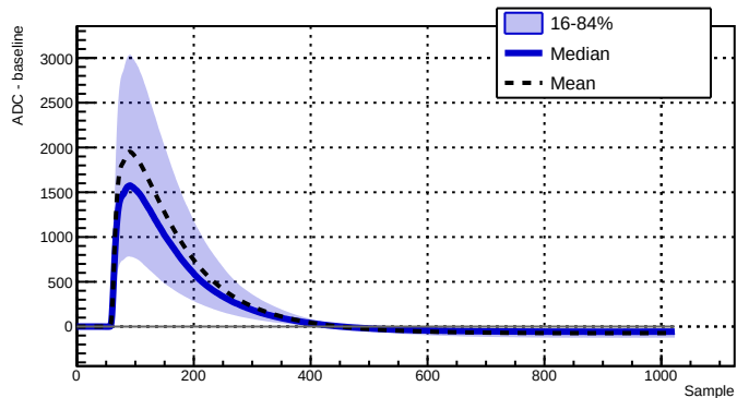
Run 039500 - Channel 2050 - 8618 waveforms
