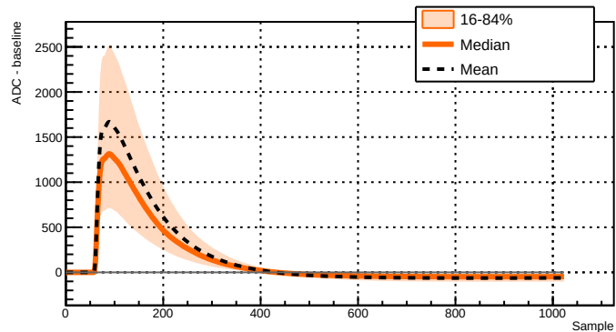
Run 039500 - Channel 2051 - 7290 waveforms
