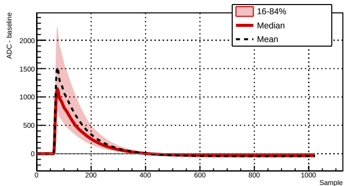
Run 039500 - Channel 2061 - 6005 waveforms
