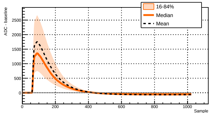
Run 039501 - Channel 2051 - 7534 waveforms
