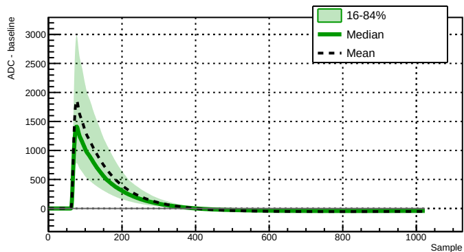
Run 039501 - Channel 2060 - 7351 waveforms
