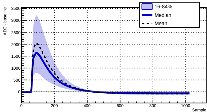
Run 039501 - Channel 2050 - 9096 waveforms
