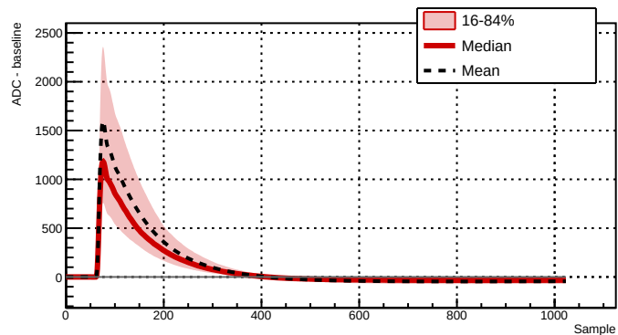
Run 039501 - Channel 2061 - 6128 waveforms
