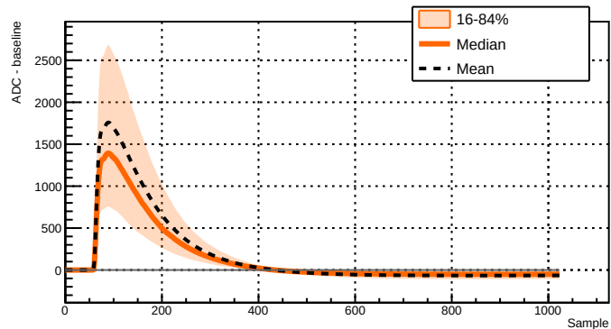
Run 039502 - Channel 2051 - 7783 waveforms
