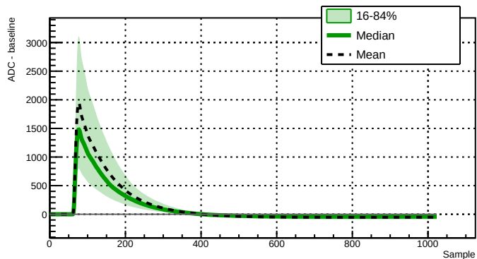
Run 039502 - Channel 2060 - 7677 waveforms
