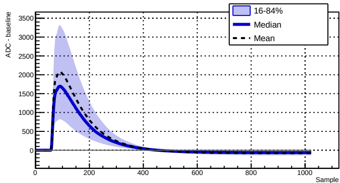
Run 039502 - Channel 2050 - 9405 waveforms
