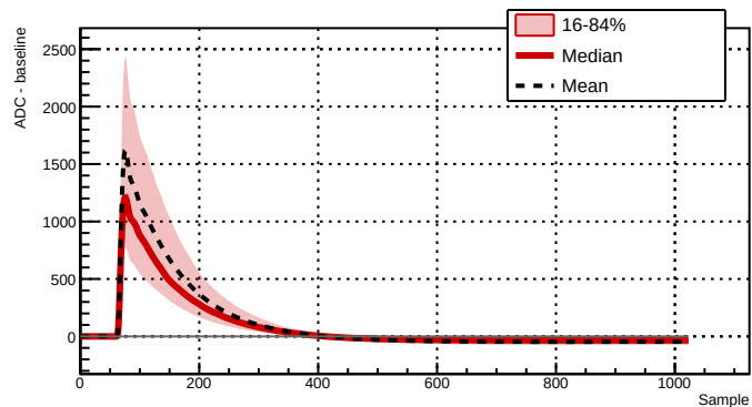
Run 039502 - Channel 2061 - 6157 waveforms
