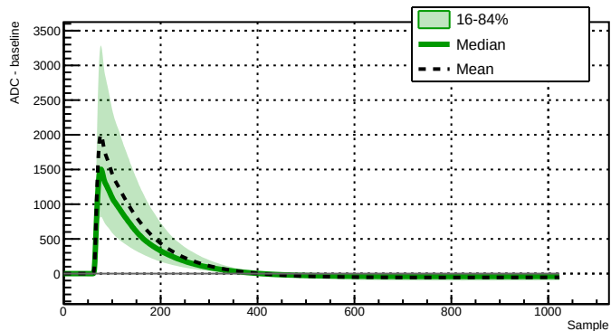
Run 039503 - Channel 2060 - 8059 waveforms
