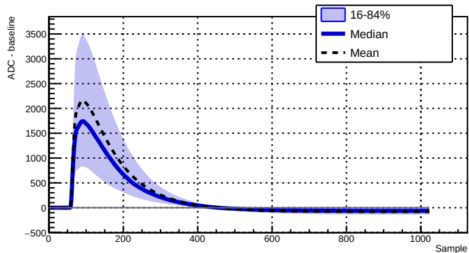
Run 039503 - Channel 2050 - 10067 waveforms
