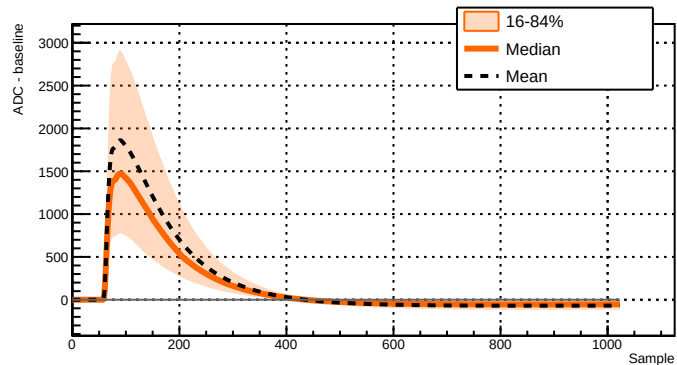
Run 039503 - Channel 2051 - 8122 waveforms
