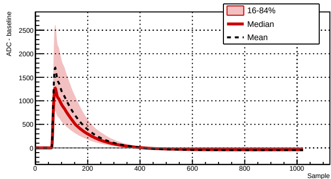
Run 039503 - Channel 2061 - 6474 waveforms
