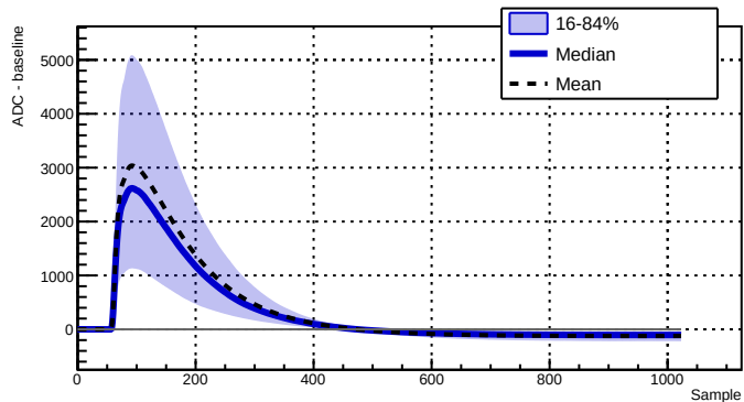
Run 039510 - Channel 2050 - 12352 waveforms
