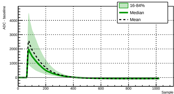
Run 039510 - Channel 2060 - 8283 waveforms
