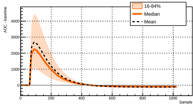
Run 039510 - Channel 2051 - 10230 waveforms
