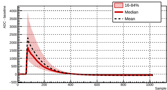
Run 039510 - Channel 2061 - 6382 waveforms
