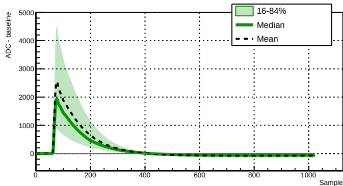
Run 039511 - Channel 2060 - 9733 waveforms
