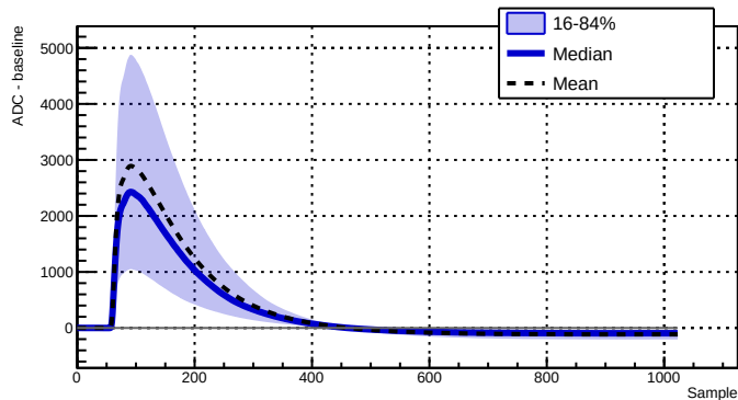
Run 039511 - Channel 2050 - 13282 waveforms
