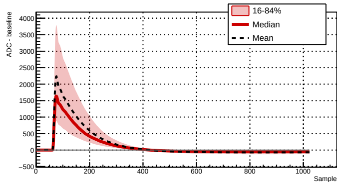
Run 039511 - Channel 2061 - 7444 waveforms
