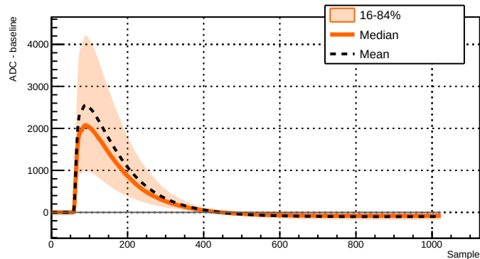
Run 039511 - Channel 2051 - 10930 waveforms
