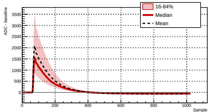
Run 039514 - Channel 2061 - 7420 waveforms
