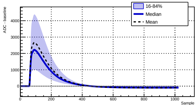
Run 039514 - Channel 2050 - 12265 waveforms
