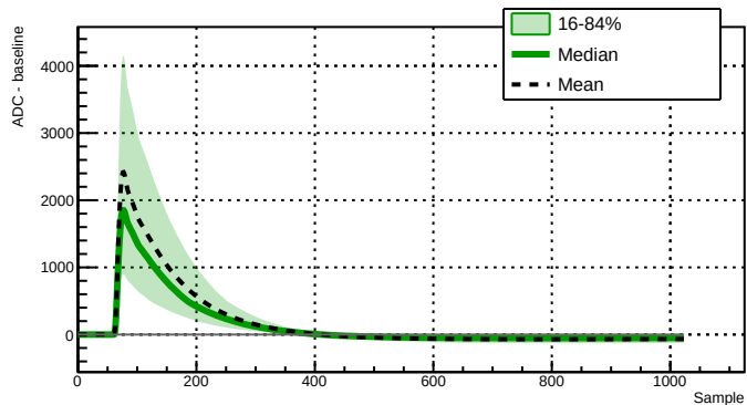
Run 039514 - Channel 2060 - 8951 waveforms
