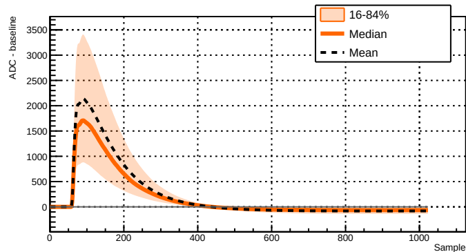
Run 039516 - Channel 2051 - 9318 waveforms
