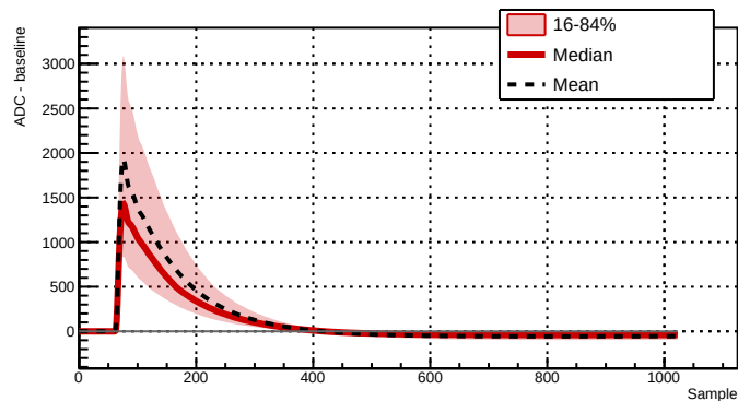
Run 039516 - Channel 2061 - 6998 waveforms
