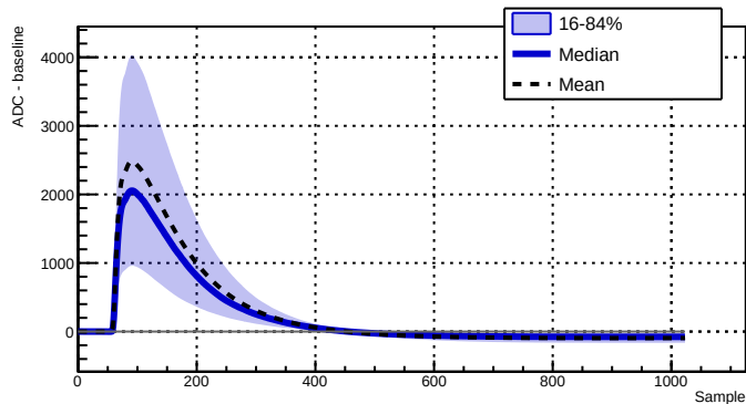
Run 039516 - Channel 2050 - 11315 waveforms
