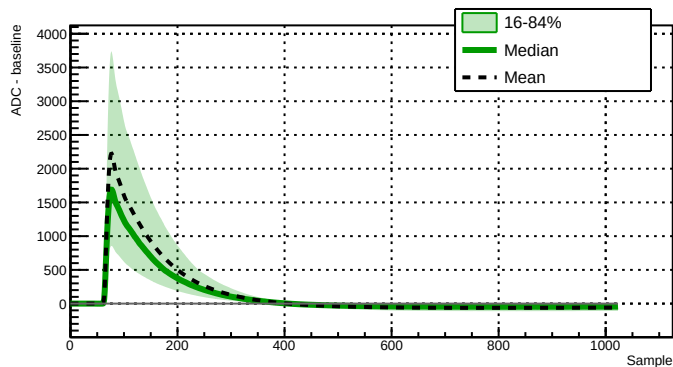
Run 039517 - Channel 2060 - 8831 waveforms
