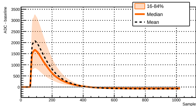
Run 039517 - Channel 2051 - 9168 waveforms
