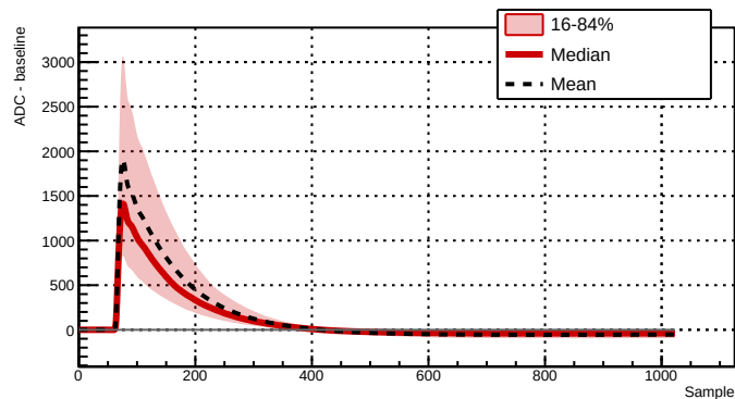
Run 039517 - Channel 2061 - 7033 waveforms
