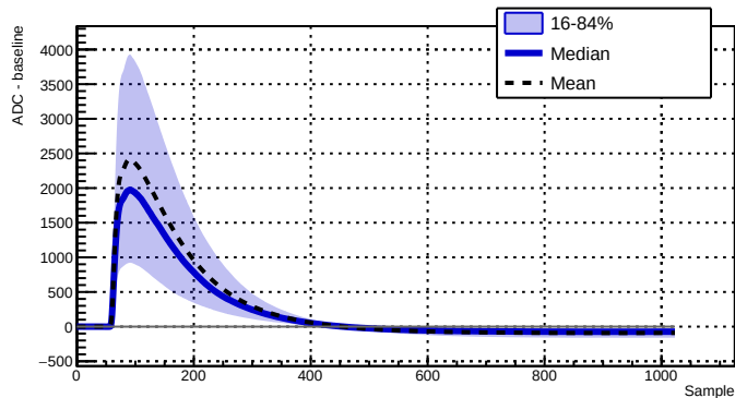
Run 039517 - Channel 2050 - 11295 waveforms
