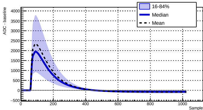
Run 039518 - Channel 2050 - 10753 waveforms
