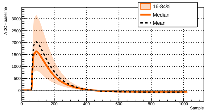
Run 039518 - Channel 2051 - 8905 waveforms
