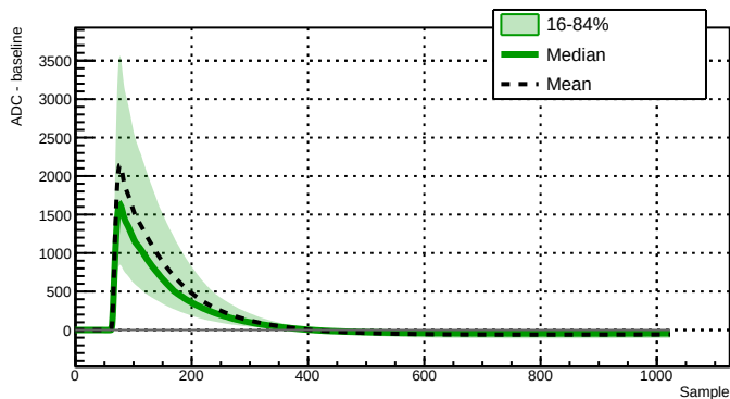
Run 039518 - Channel 2060 - 8473 waveforms
