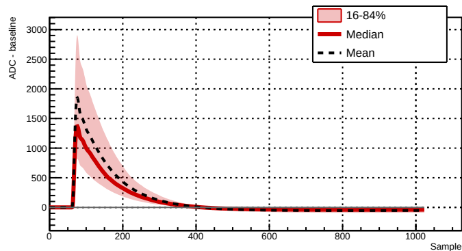
Run 039518 - Channel 2061 - 6795 waveforms
