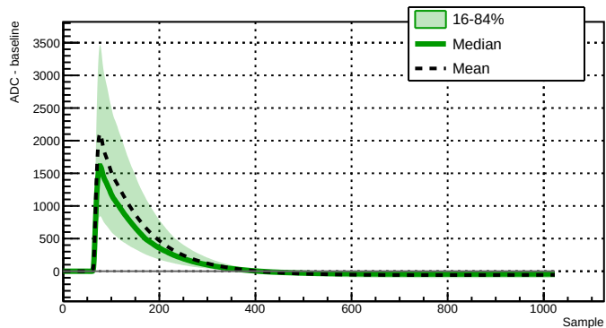
Run 039519 - Channel 2060 - 8275 waveforms
