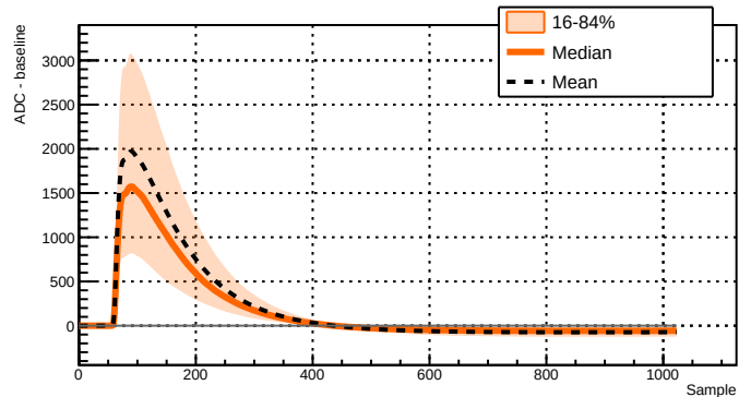
Run 039519 - Channel 2051 - 8763 waveforms
