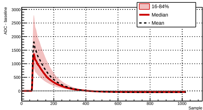
Run 039519 - Channel 2061 - 6731 waveforms
