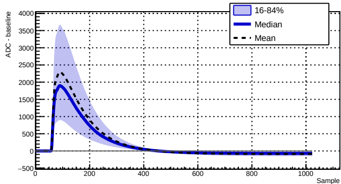
Run 039519 - Channel 2050 - 10459 waveforms
