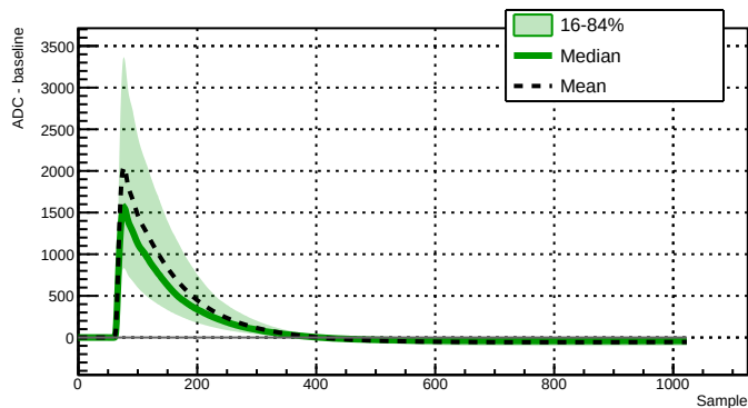
Run 039521 - Channel 2060 - 8125 waveforms
