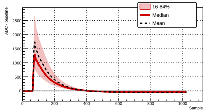
Run 039521 - Channel 2061 - 6591 waveforms
