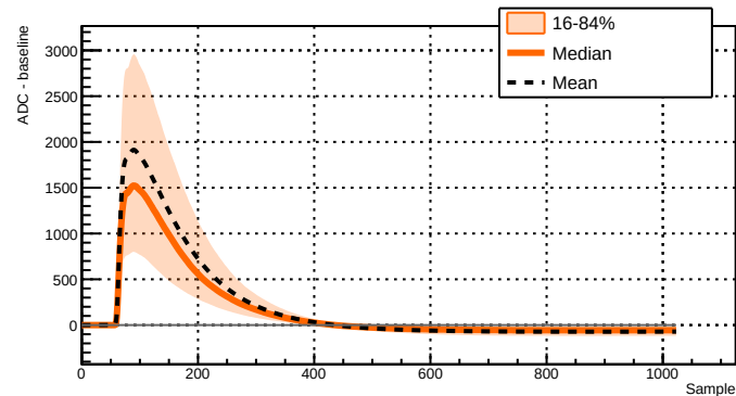
Run 039521 - Channel 2051 - 8388 waveforms
