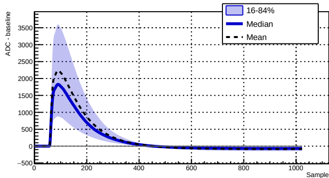
Run 039521 - Channel 2050 - 10213 waveforms
