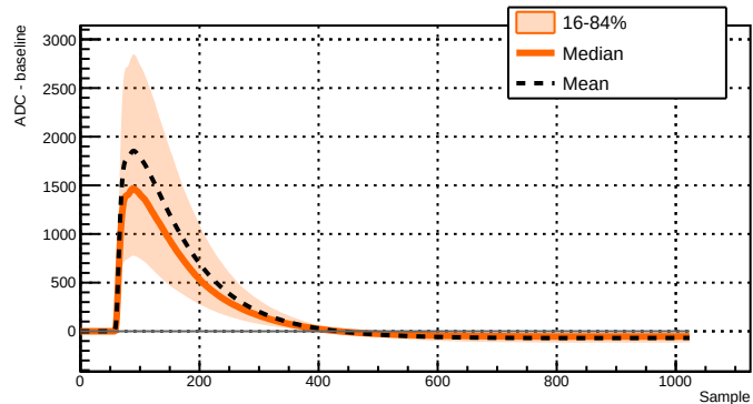
Run 039522 - Channel 2051 - 8137 waveforms
