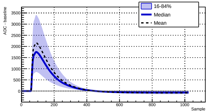
Run 039522 - Channel 2050 - 9889 waveforms
