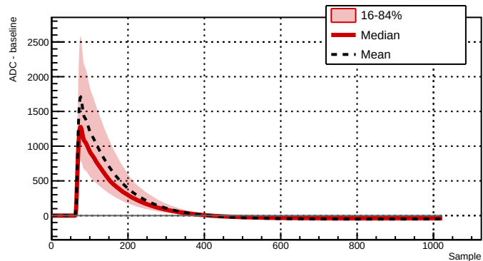
Run 039522 - Channel 2061 - 6374 waveforms
