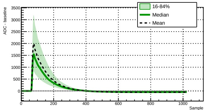
Run 039522 - Channel 2060 - 7909 waveforms
