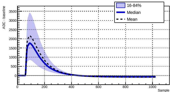
Run 039523 - Channel 2050 - 9671 waveforms
