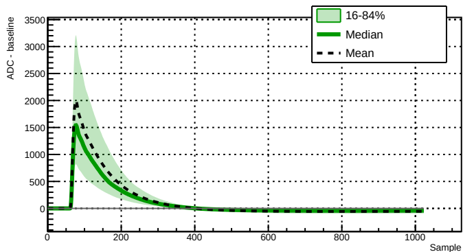
Run 039523 - Channel 2060 - 7807 waveforms
