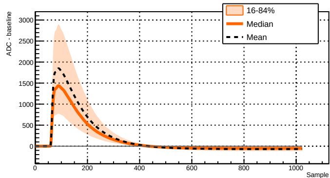
Run 039523 - Channel 2051 - 7842 waveforms
