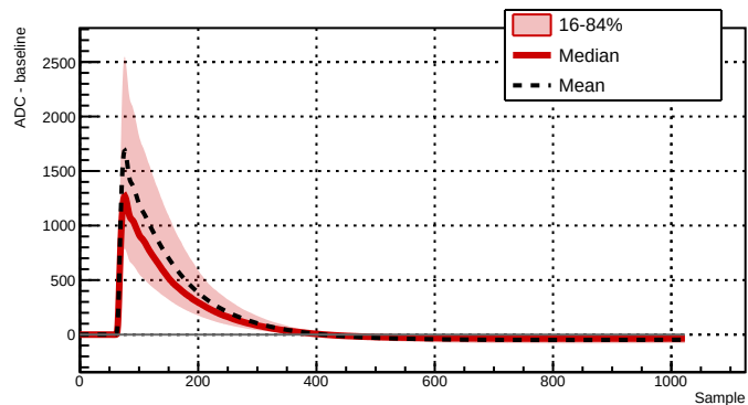
Run 039523 - Channel 2061 - 6490 waveforms
