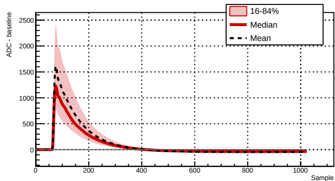
Run 039526 - Channel 2061 - 6234 waveforms
