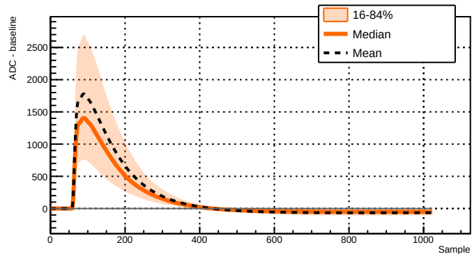
Run 039526 - Channel 2051 - 7617 waveforms
