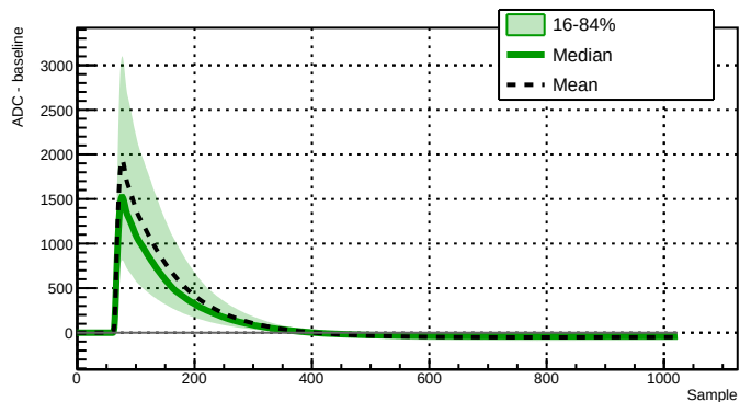
Run 039526 - Channel 2060 - 7504 waveforms
