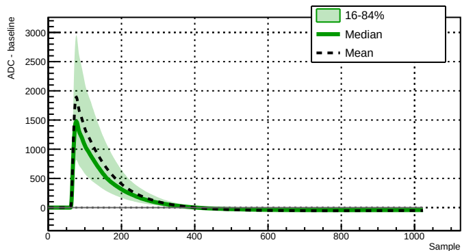
Run 039527 - Channel 2060 - 7389 waveforms
