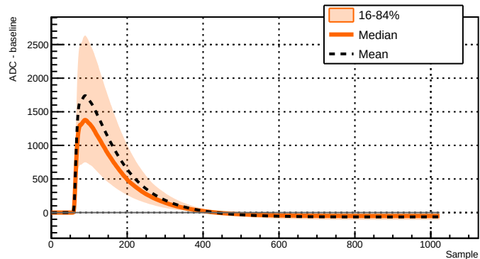
Run 039527 - Channel 2051 - 7465 waveforms
