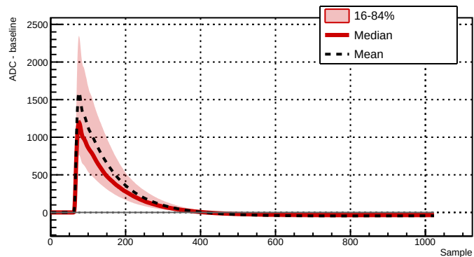
Run 039527 - Channel 2061 - 6073 waveforms
