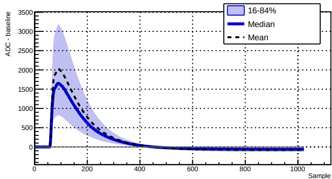
Run 039527 - Channel 2050 - 9099 waveforms
