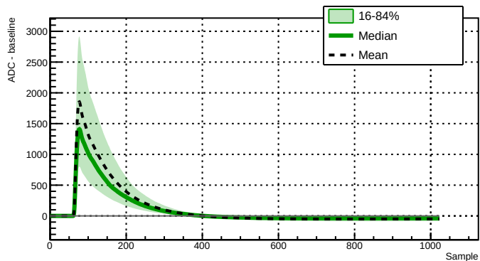
Run 039528 - Channel 2060 - 7371 waveforms
