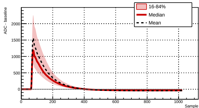
Run 039528 - Channel 2061 - 5963 waveforms
