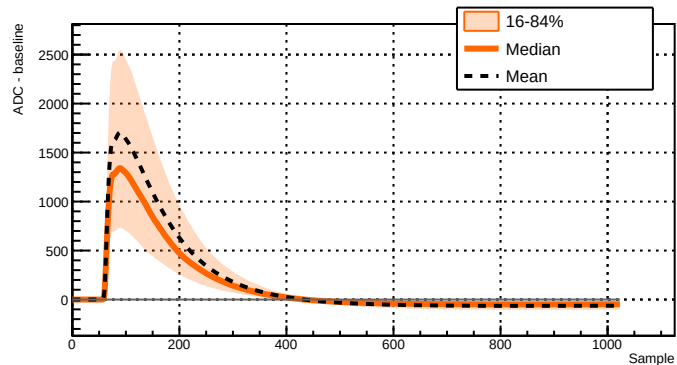
Run 039528 - Channel 2051 - 7330 waveforms
