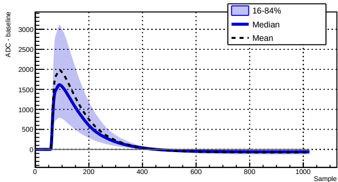
Run 039528 - Channel 2050 - 9025 waveforms
