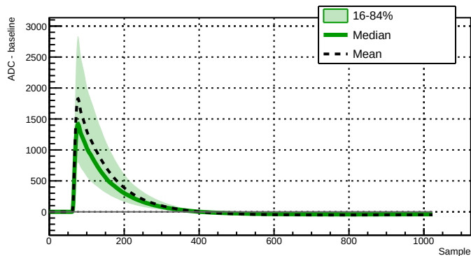
Run 039529 - Channel 2060 - 7168 waveforms
