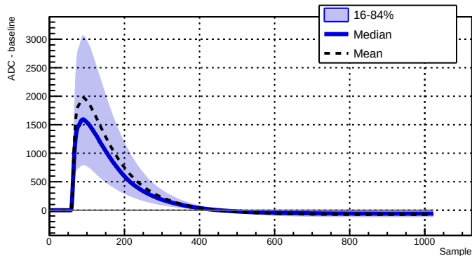
Run 039529 - Channel 2050 - 8782 waveforms
