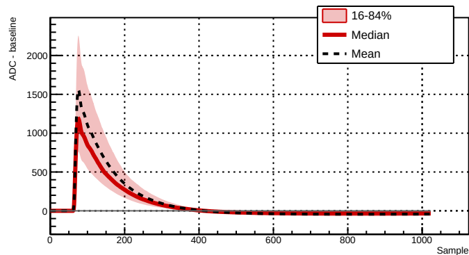
Run 039529 - Channel 2061 - 5880 waveforms
