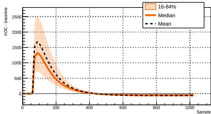
Run 039529 - Channel 2051 - 7197 waveforms
