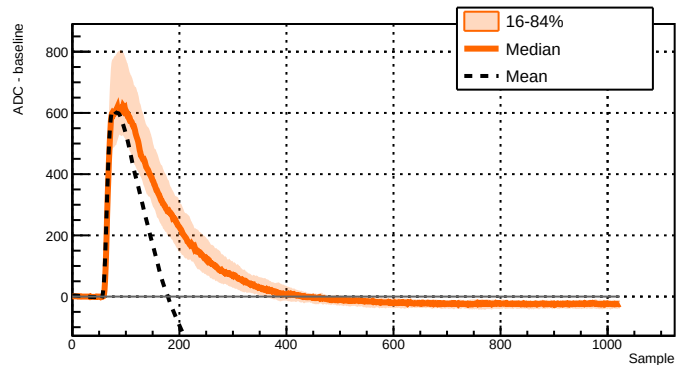
Run 040931 - Channel 2051 - 99 waveforms
