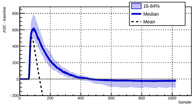
Run 040931 - Channel 2050 - 127 waveforms
