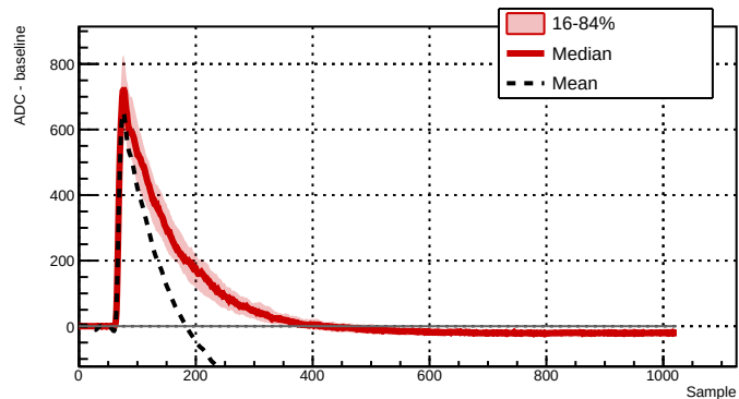
Run 040931 - Channel 2061 - 99 waveforms
