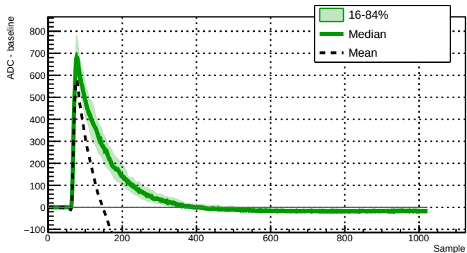
Run 040931 - Channel 2060 - 99 waveforms
