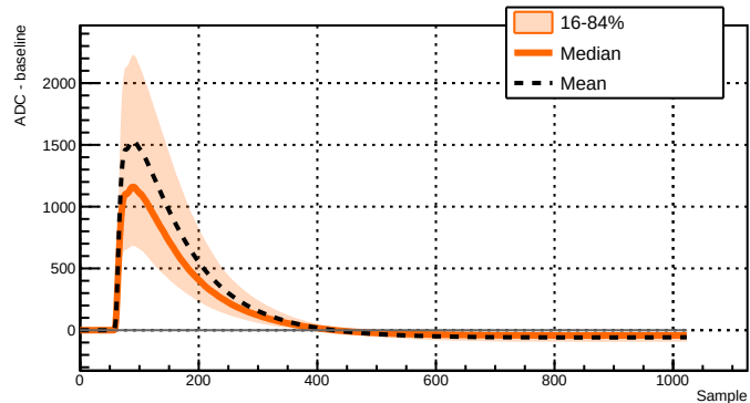
Run 043381 - Channel 2051 - 6108 waveforms
