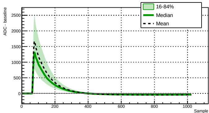
Run 043381 - Channel 2060 - 6274 waveforms
