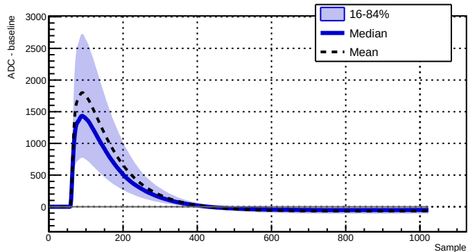
Run 043381 - Channel 2050 - 7538 waveforms
