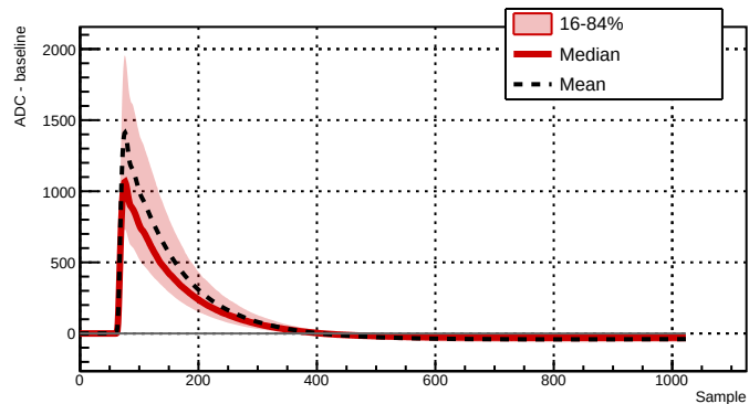
Run 043381 - Channel 2061 - 5286 waveforms
