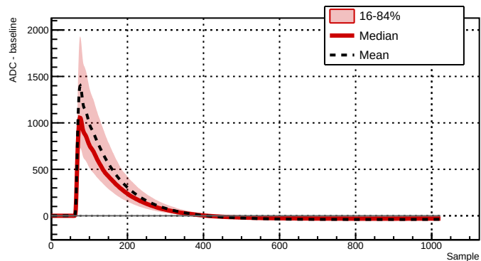
Run 043386 - Channel 2061 - 5110 waveforms
