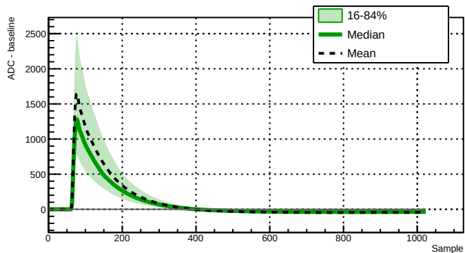
Run 043386 - Channel 2060 - 6202 waveforms
