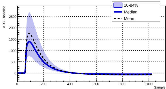
Run 043386 - Channel 2050 - 7472 waveforms
