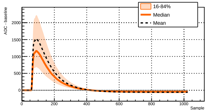
Run 043386 - Channel 2051 - 5850 waveforms
