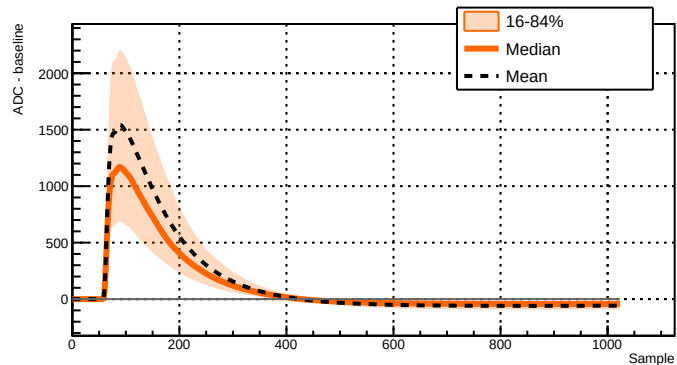
Run 043387 - Channel 2051 - 5878 waveforms
