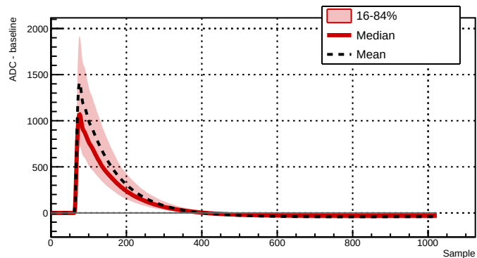
Run 043387 - Channel 2061 - 5173 waveforms
