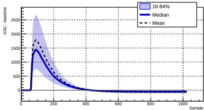
Run 043387 - Channel 2050 - 7263 waveforms
