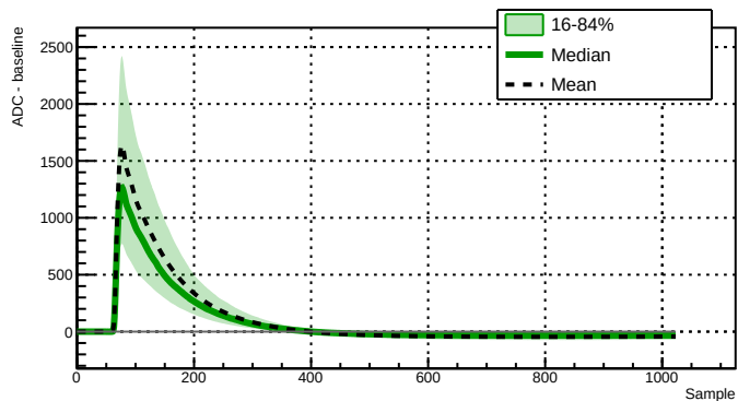
Run 043387 - Channel 2060 - 6253 waveforms
