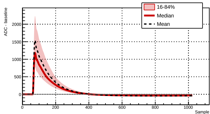
Run 043389 - Channel 2061 - 5672 waveforms
