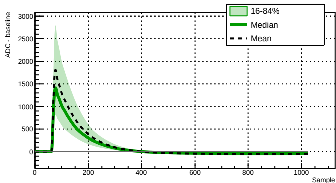
Run 043389 - Channel 2060 - 6992 waveforms
