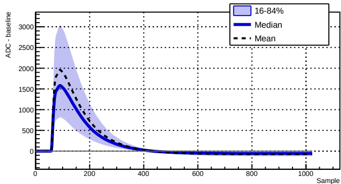
Run 043389 - Channel 2050 - 8787 waveforms
