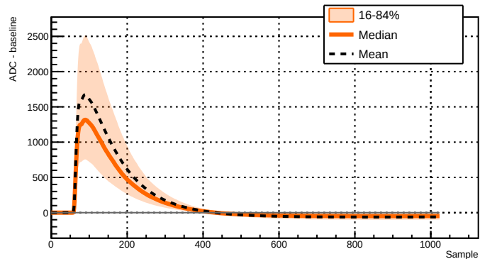
Run 043389 - Channel 2051 - 6924 waveforms
