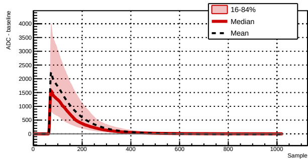
Run 039500 - Channel 1021 - 2907 waveforms
