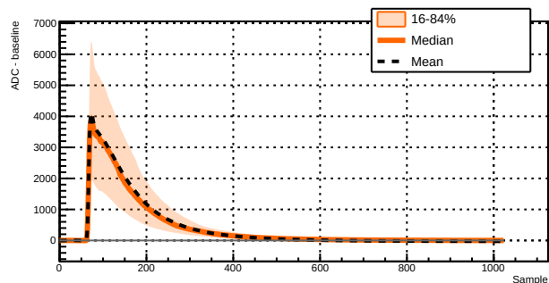
Run 039500 - Channel 1071 - 1547 waveforms
