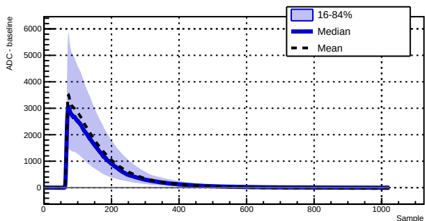
Run 039500 - Channel 1070 - 1543 waveforms
