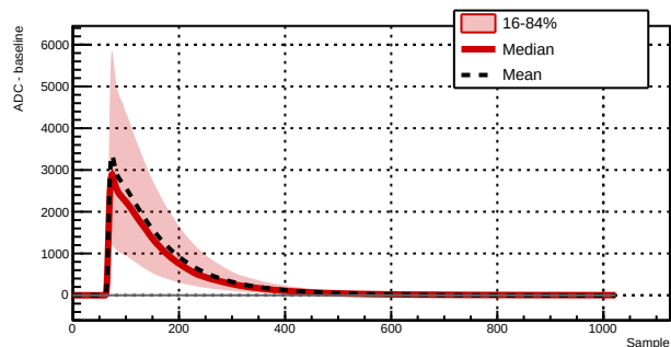
Run 039500 - Channel 1061 - 8427 waveforms
