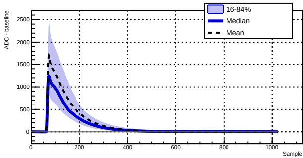
Run 039500 - Channel 1010 - 6024 waveforms
