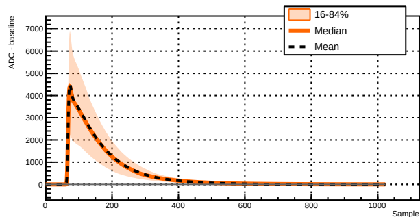
Run 039500 - Channel 1031 - 4985 waveforms
