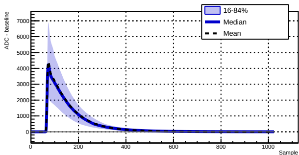
Run 039500 - Channel 1030 - 4311 waveforms
