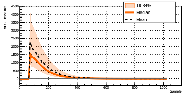
Run 039500 - Channel 1011 - 17116 waveforms
