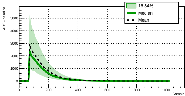
Run 039500 - Channel 1020 - 12336 waveforms
