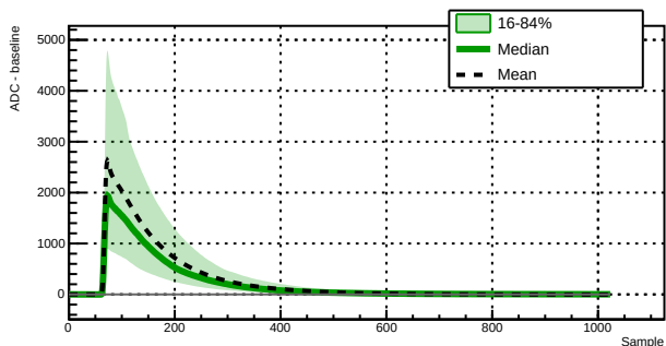
Run 039500 - Channel 1060 - 8817 waveforms
