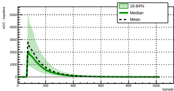
Run 039501 - Channel 1060 - 9351 waveforms
