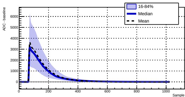
Run 039501 - Channel 1070 - 1514 waveforms
