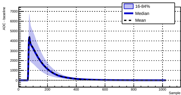
Run 039501 - Channel 1030 - 4171 waveforms
