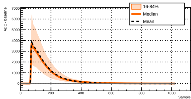
Run 039501 - Channel 1071 - 1444 waveforms
