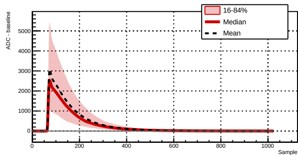
Run 039501 - Channel 1061 - 6735 waveforms
