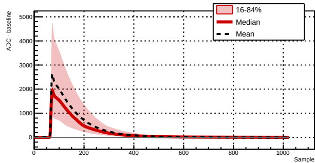
Run 039501 - Channel 1021 - 4183 waveforms
