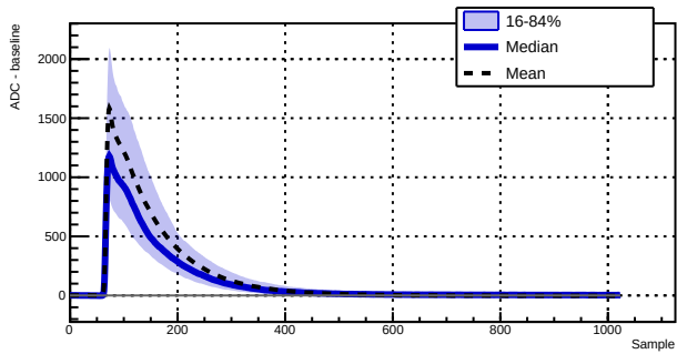
Run 039501 - Channel 1010 - 5694 waveforms
