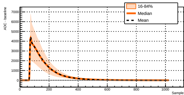
Run 039501 - Channel 1031 - 4454 waveforms
