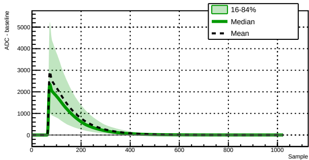
Run 039501 - Channel 1020 - 13460 waveforms
