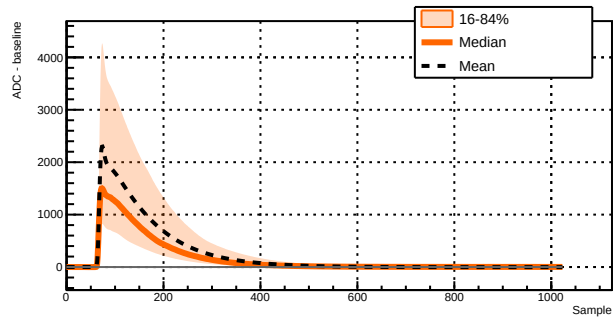
Run 039501 - Channel 1011 - 14242 waveforms
