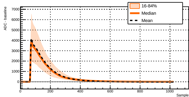
Run 039502 - Channel 1071 - 1610 waveforms
