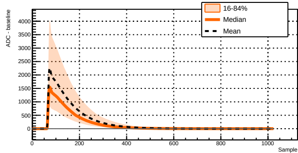
Run 039502 - Channel 1011 - 15721 waveforms
