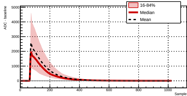
Run 039502 - Channel 1021 - 4640 waveforms
