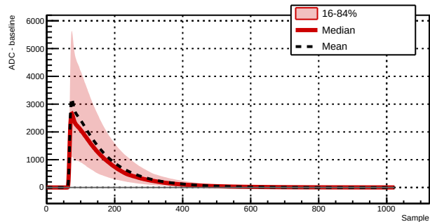
Run 039502 - Channel 1061 - 7350 waveforms
