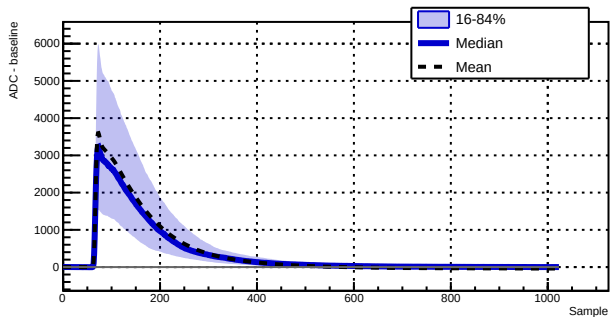
Run 039502 - Channel 1070 - 1438 waveforms
