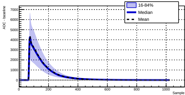
Run 039502 - Channel 1030 - 4225 waveforms
