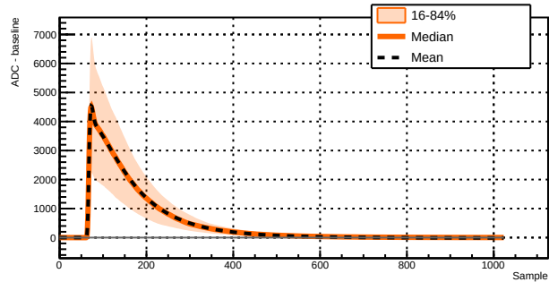
Run 039502 - Channel 1031 - 3881 waveforms
