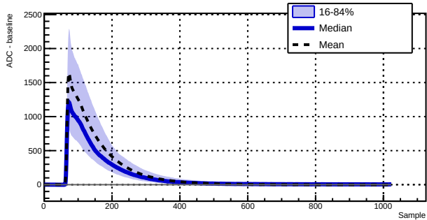
Run 039502 - Channel 1010 - 6035 waveforms
