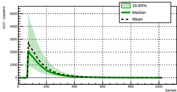
Run 039502 - Channel 1060 - 9774 waveforms
