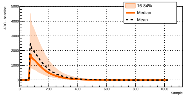
Run 039504 - Channel 1011 - 16950 waveforms
