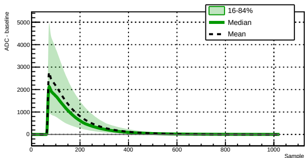
Run 039504 - Channel 1060 - 9715 waveforms
