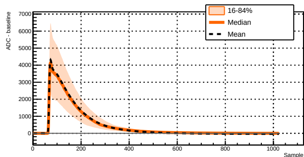
Run 039504 - Channel 1071 - 1703 waveforms
