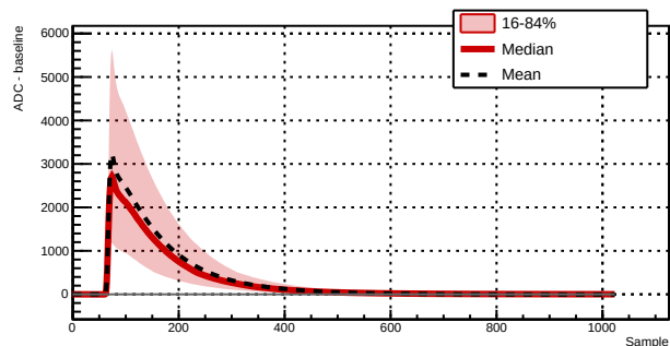
Run 039504 - Channel 1061 - 7782 waveforms
