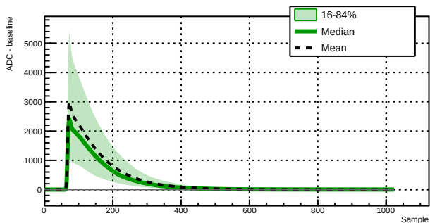
Run 039504 - Channel 1020 - 12862 waveforms
