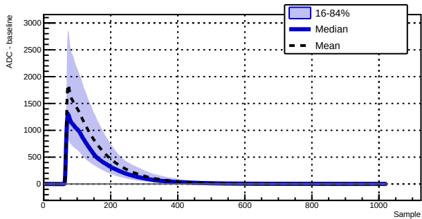
Run 039504 - Channel 1010 - 6753 waveforms
