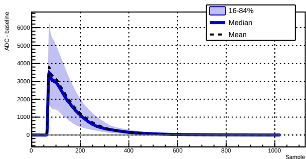
Run 039504 - Channel 1070 - 1376 waveforms
