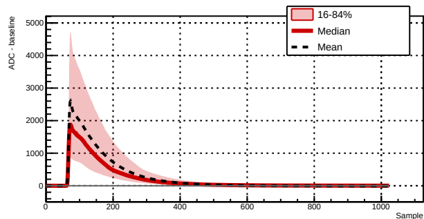
Run 039504 - Channel 1021 - 4548 waveforms
