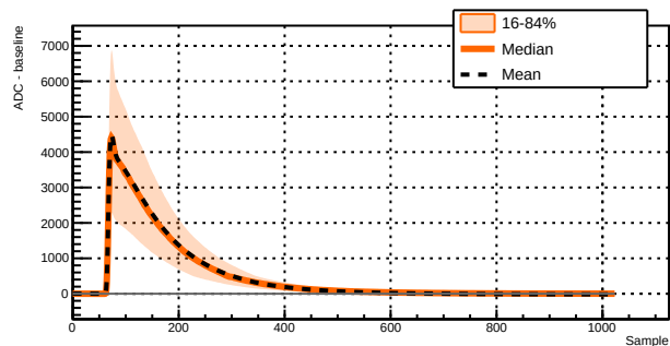
Run 039504 - Channel 1031 - 2874 waveforms
