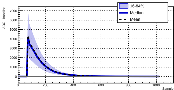
Run 039504 - Channel 1030 - 3931 waveforms
