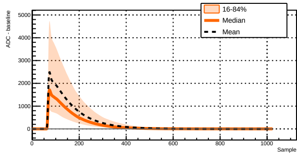
Run 039506 - Channel 1011 - 17061 waveforms
