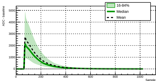
Run 039506 - Channel 1060 - 9255 waveforms
