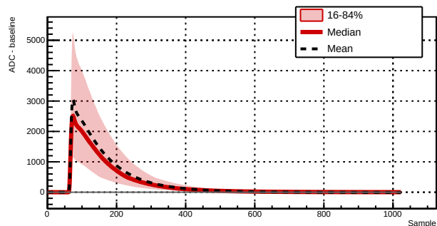
Run 039506 - Channel 1061 - 6995 waveforms
