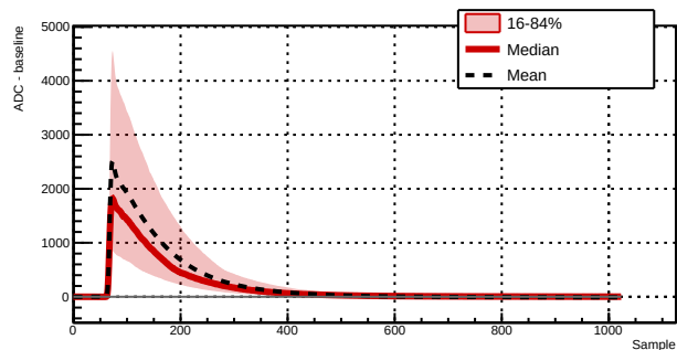
Run 039506 - Channel 1021 - 3980 waveforms
