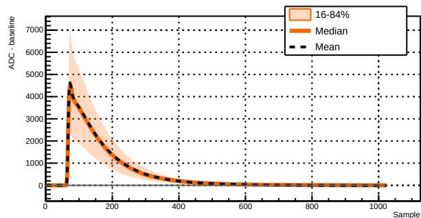
Run 039506 - Channel 1031 - 4620 waveforms
