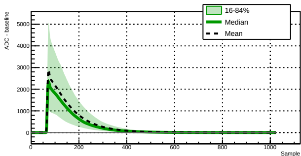
Run 039506 - Channel 1020 - 12094 waveforms
