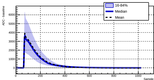
Run 039506 - Channel 1070 - 1578 waveforms
