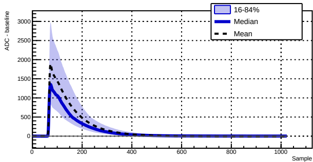
Run 039506 - Channel 1010 - 6823 waveforms
