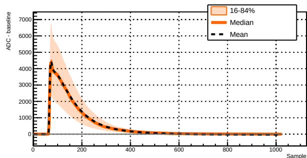
Run 039506 - Channel 1071 - 1678 waveforms
