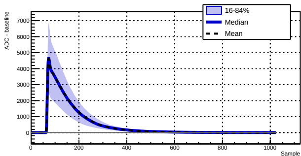
Run 039506 - Channel 1030 - 4266 waveforms
