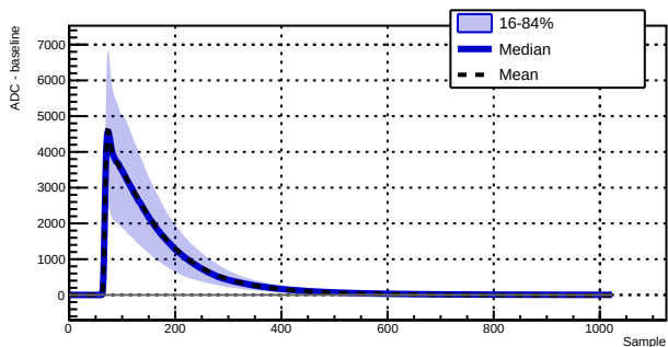
Run 039507 - Channel 1030 - 4209 waveforms
