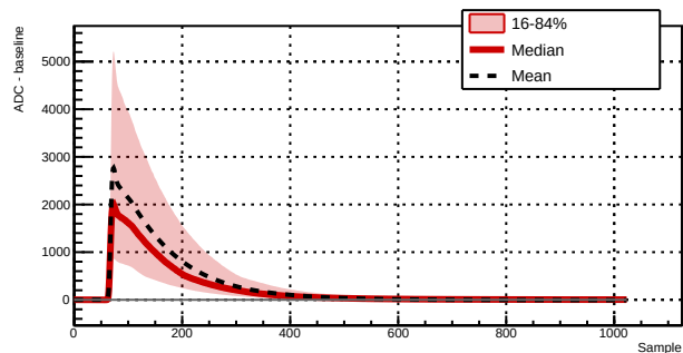
Run 039507 - Channel 1021 - 4419 waveforms
