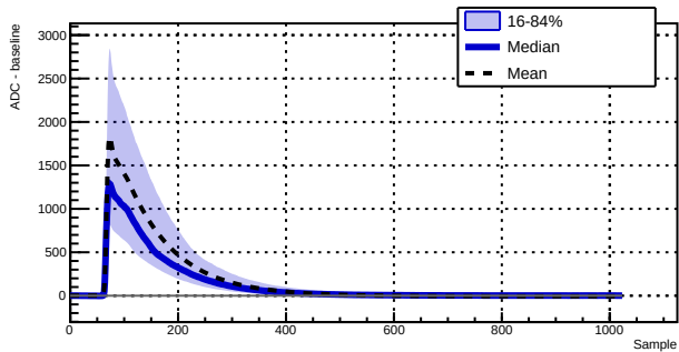
Run 039507 - Channel 1010 - 6161 waveforms
