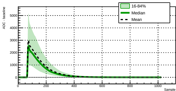
Run 039507 - Channel 1020 - 12548 waveforms
