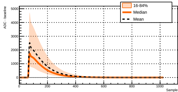
Run 039507 - Channel 1011 - 18031 waveforms
