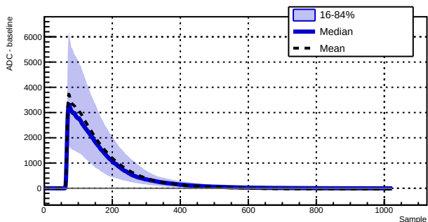
Run 039507 - Channel 1070 - 1185 waveforms
