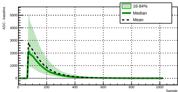
Run 039507 - Channel 1060 - 8815 waveforms
