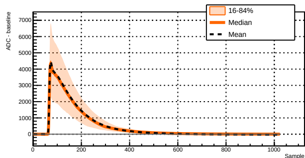
Run 039507 - Channel 1071 - 1650 waveforms
