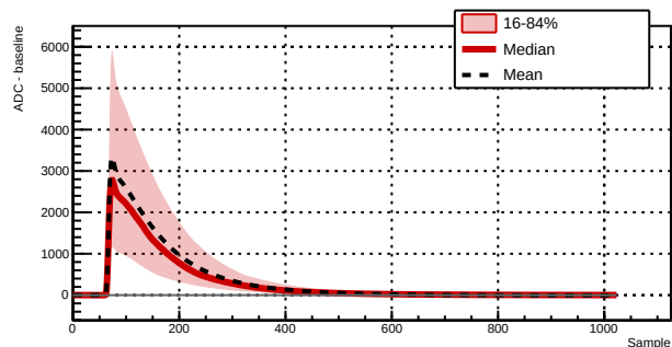
Run 039507 - Channel 1061 - 7143 waveforms
