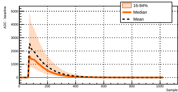
Run 039508 - Channel 1011 - 14265 waveforms
