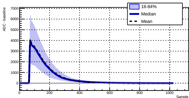
Run 039508 - Channel 1070 - 1220 waveforms
