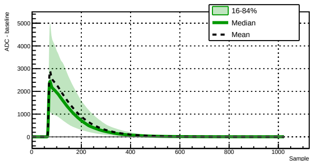
Run 039508 - Channel 1020 - 11043 waveforms
