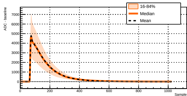
Run 039508 - Channel 1031 - 4475 waveforms
