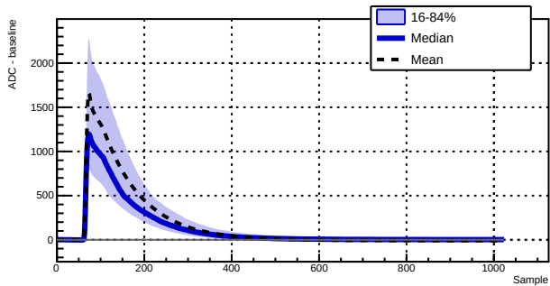
Run 039508 - Channel 1010 - 4826 waveforms
