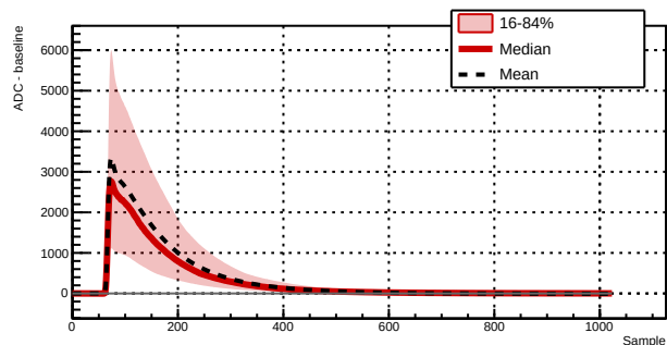
Run 039508 - Channel 1061 - 6172 waveforms
