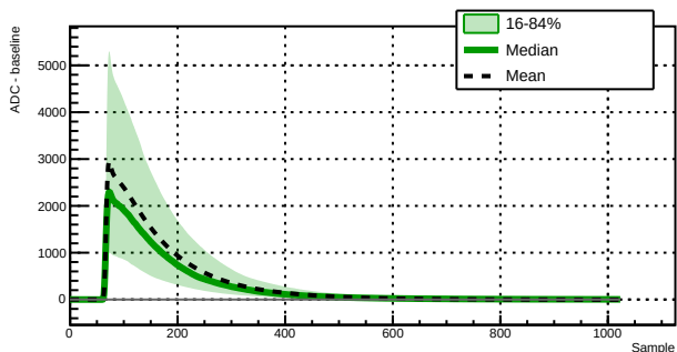
Run 039508 - Channel 1060 - 8673 waveforms
