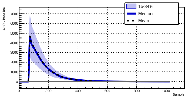
Run 039508 - Channel 1030 - 4211 waveforms
