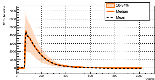
Run 039508 - Channel 1071 - 947 waveforms
