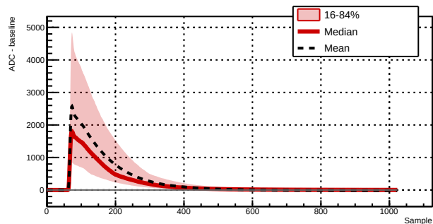
Run 039508 - Channel 1021 - 3454 waveforms
