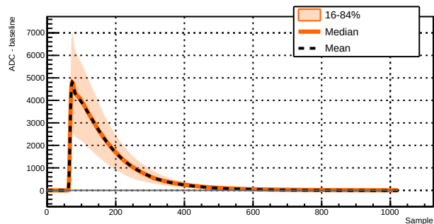
Run 039510 - Channel 1031 - 4301 waveforms
