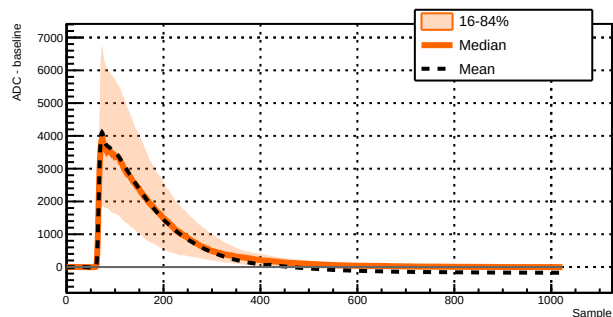
Run 039510 - Channel 1071 - 565 waveforms
