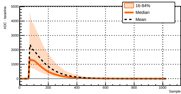
Run 039510 - Channel 1011 - 12056 waveforms
