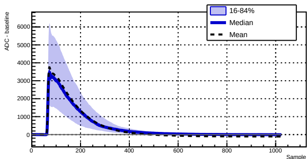
Run 039510 - Channel 1070 - 747 waveforms
