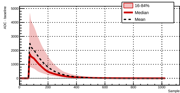
Run 039510 - Channel 1021 - 3000 waveforms
