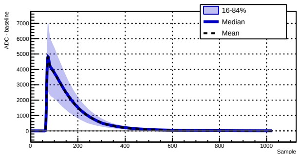
Run 039510 - Channel 1030 - 3565 waveforms
