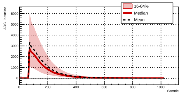
Run 039510 - Channel 1061 - 4380 waveforms
