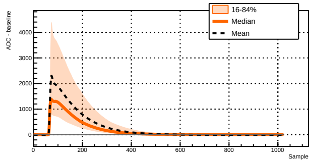
Run 039511 - Channel 1011 - 13830 waveforms
