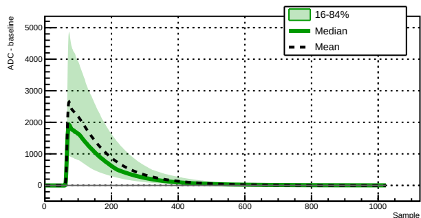
Run 039511 - Channel 1060 - 6799 waveforms
