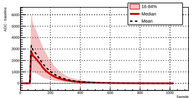
Run 039511 - Channel 1061 - 5334 waveforms
