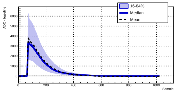
Run 039511 - Channel 1070 - 859 waveforms
