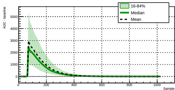
Run 039511 - Channel 1020 - 10918 waveforms
