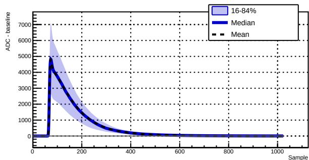
Run 039511 - Channel 1030 - 4196 waveforms
