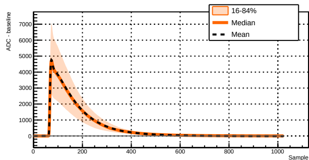
Run 039511 - Channel 1031 - 3957 waveforms
