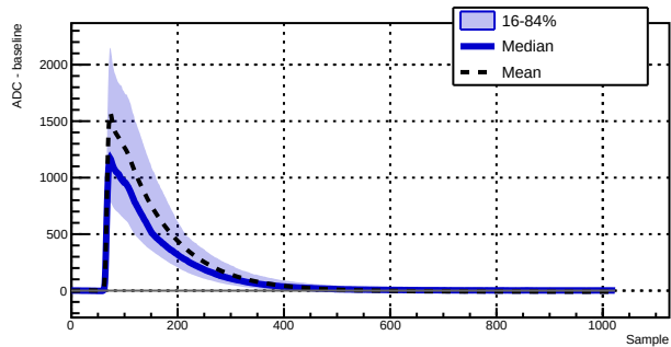
Run 039511 - Channel 1010 - 4280 waveforms
