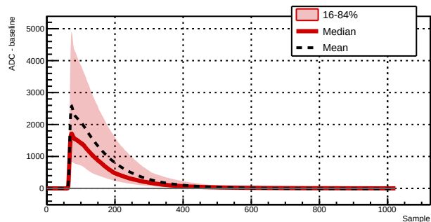
Run 039511 - Channel 1021 - 3095 waveforms
