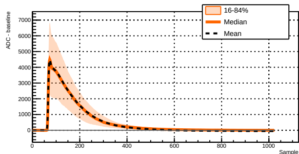
Run 039511 - Channel 1071 - 861 waveforms
