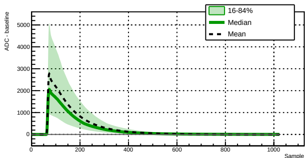
Run 039515 - Channel 1060 - 8591 waveforms
