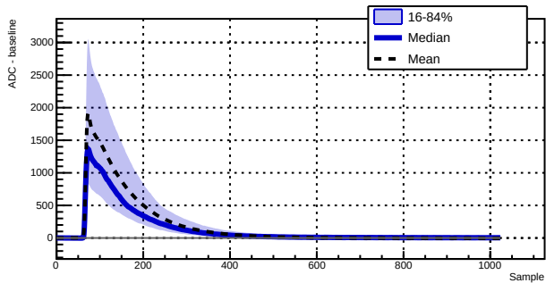
Run 039515 - Channel 1010 - 5877 waveforms
