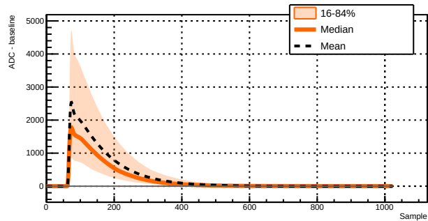
Run 039515 - Channel 1011 - 16211 waveforms
