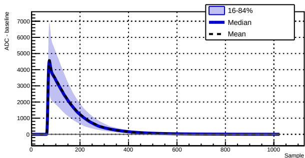
Run 039515 - Channel 1030 - 3988 waveforms
