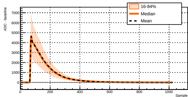
Run 039515 - Channel 1031 - 4804 waveforms
