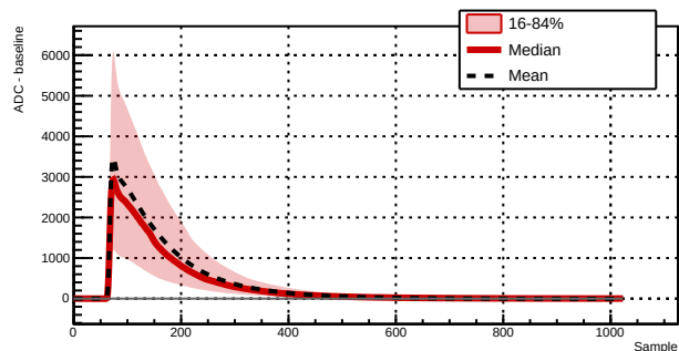
Run 039515 - Channel 1061 - 7259 waveforms
