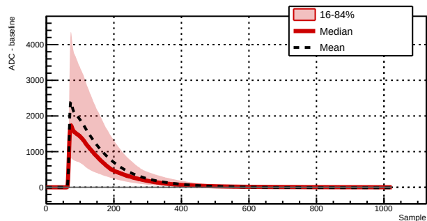
Run 039515 - Channel 1021 - 3802 waveforms
