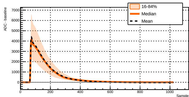
Run 039515 - Channel 1071 - 1189 waveforms
