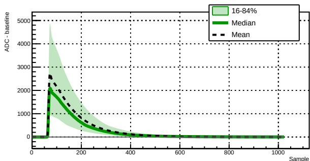
Run 039516 - Channel 1060 - 9253 waveforms
