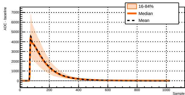
Run 039516 - Channel 1031 - 4646 waveforms
