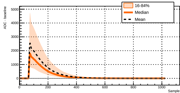
Run 039516 - Channel 1011 - 16318 waveforms
