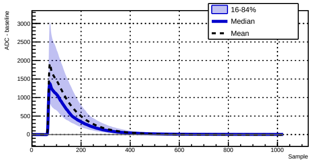
Run 039516 - Channel 1010 - 6272 waveforms
