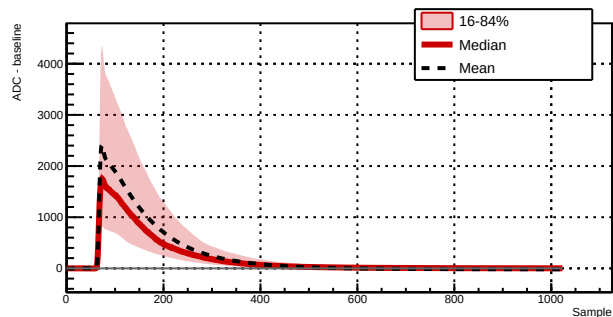
Run 039516 - Channel 1021 - 3139 waveforms
