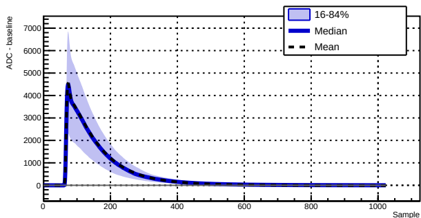
Run 039516 - Channel 1030 - 4284 waveforms
