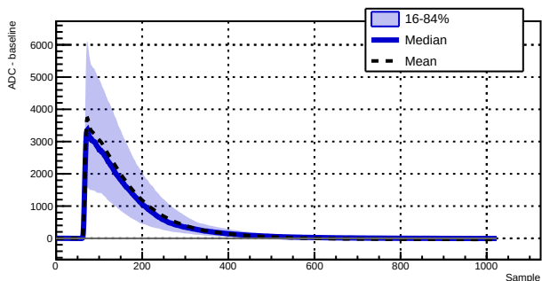
Run 039516 - Channel 1070 - 1305 waveforms
