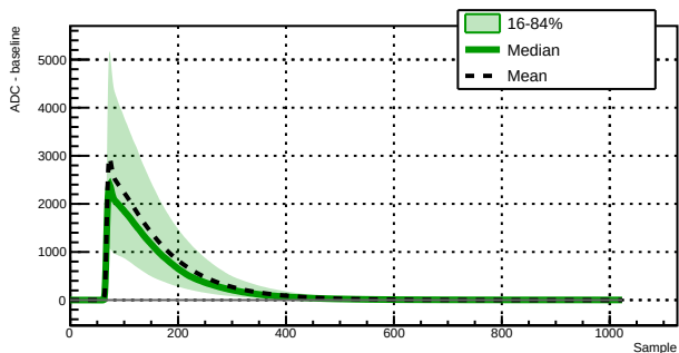
Run 039516 - Channel 1020 - 12733 waveforms
