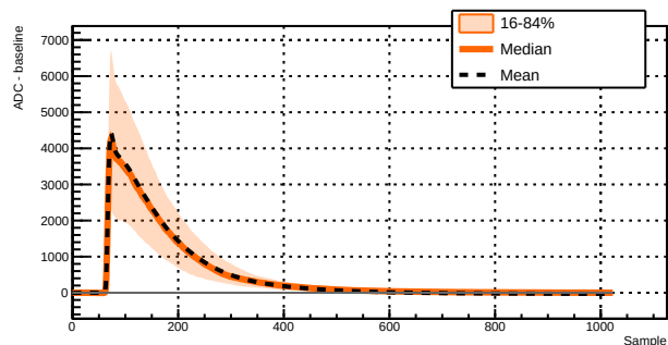
Run 039516 - Channel 1071 - 1316 waveforms
