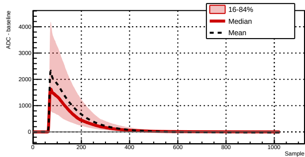
Run 039517 - Channel 1021 - 2806 waveforms
