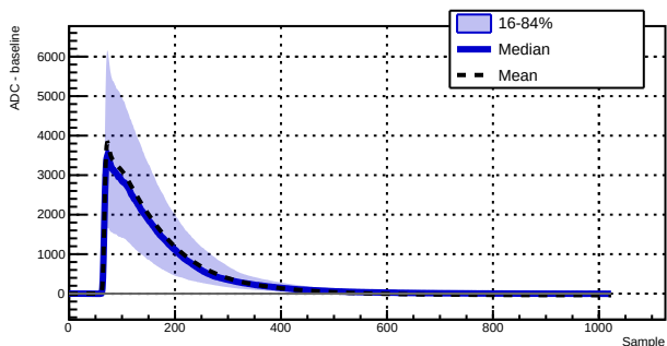
Run 039517 - Channel 1070 - 1427 waveforms
