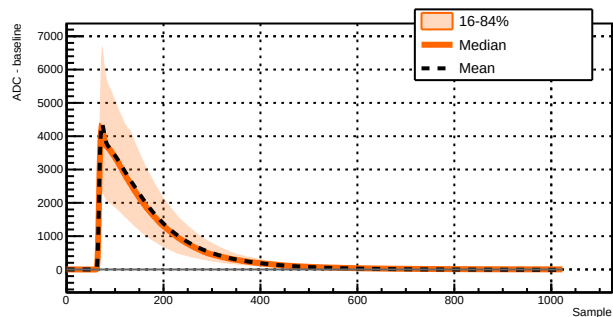
Run 039517 - Channel 1031 - 4070 waveforms
