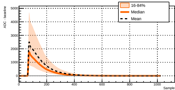
Run 039517 - Channel 1011 - 15138 waveforms
