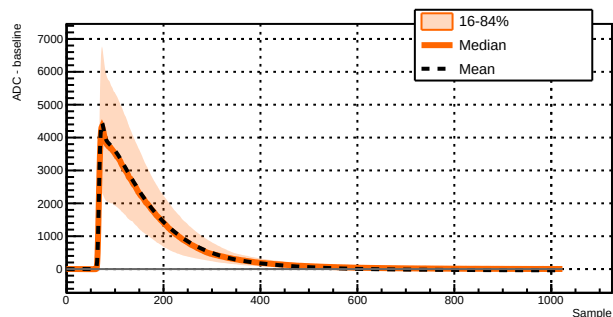
Run 039517 - Channel 1071 - 1436 waveforms
