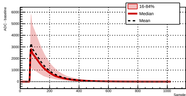
Run 039517 - Channel 1061 - 7126 waveforms
