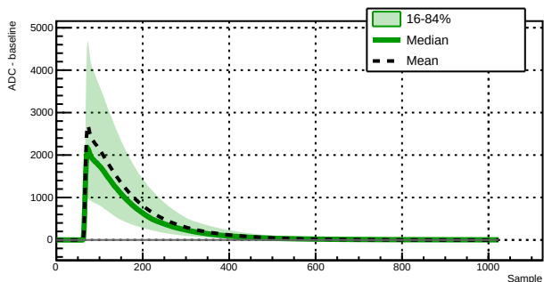
Run 039517 - Channel 1060 - 9872 waveforms
