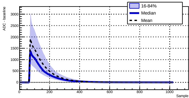
Run 039517 - Channel 1010 - 6954 waveforms
