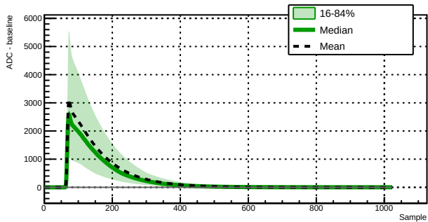
Run 039517 - Channel 1020 - 13303 waveforms
