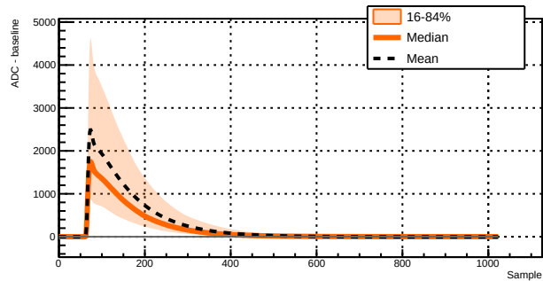
Run 039519 - Channel 1011 - 16007 waveforms
