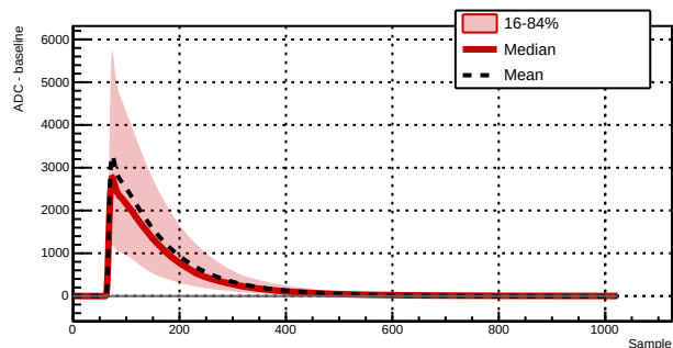
Run 039519 - Channel 1061 - 7444 waveforms
