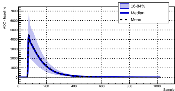
Run 039519 - Channel 1030 - 4145 waveforms
