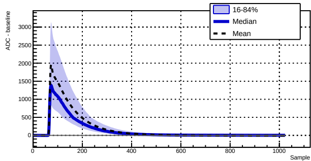
Run 039519 - Channel 1010 - 6568 waveforms
