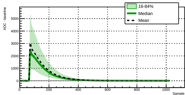
Run 039519 - Channel 1020 - 13624 waveforms
