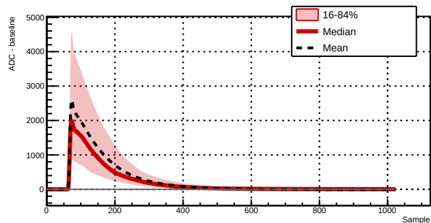
Run 039519 - Channel 1021 - 5019 waveforms
