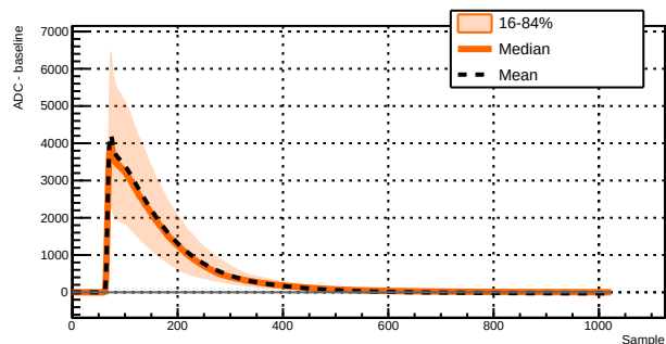
Run 039519 - Channel 1071 - 1712 waveforms
