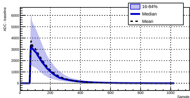
Run 039519 - Channel 1070 - 1545 waveforms
