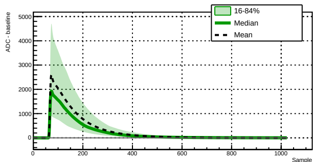
Run 039519 - Channel 1060 - 8583 waveforms
