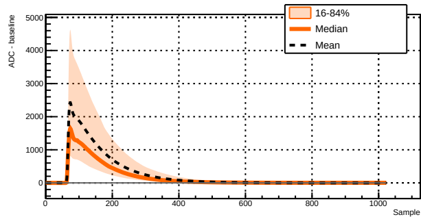
Run 039521 - Channel 1011 - 15653 waveforms
