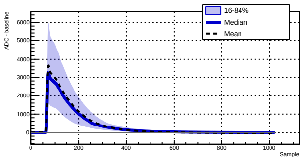
Run 039521 - Channel 1070 - 1525 waveforms
