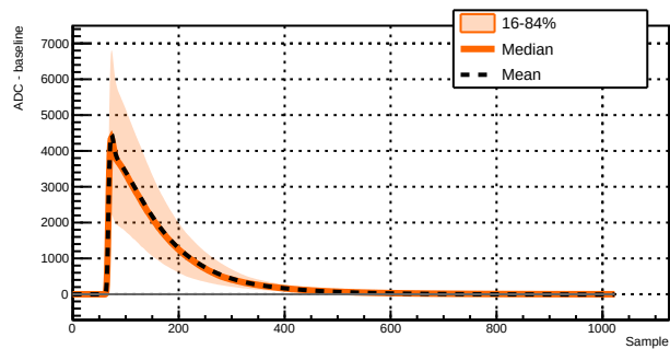
Run 039521 - Channel 1031 - 6309 waveforms
