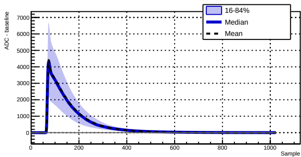
Run 039521 - Channel 1030 - 4446 waveforms
