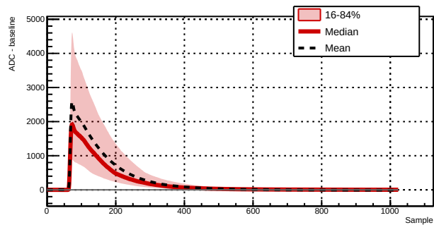
Run 039521 - Channel 1021 - 4110 waveforms
