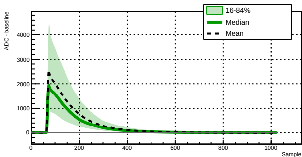
Run 039521 - Channel 1060 - 8745 waveforms
