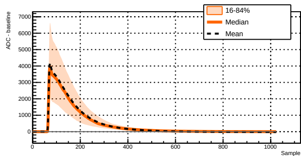
Run 039521 - Channel 1071 - 1717 waveforms
