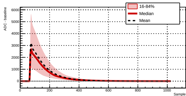
Run 039521 - Channel 1061 - 7728 waveforms
